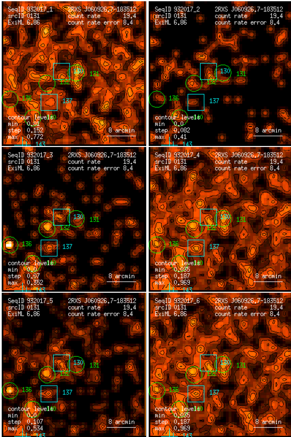
Figure 131: RASS 932017: detection 0131: band rate images, Gaussian filter: (1) PSPC channels 11 – 41, (2) 52 – 90, (3) 91 – 201, (4) 11 – 235, (5) 52 – 201, (6) 11 – 201. Broad band rates in counts/ks. Band rate contour levels in counts/ks/arcmin 2 .
