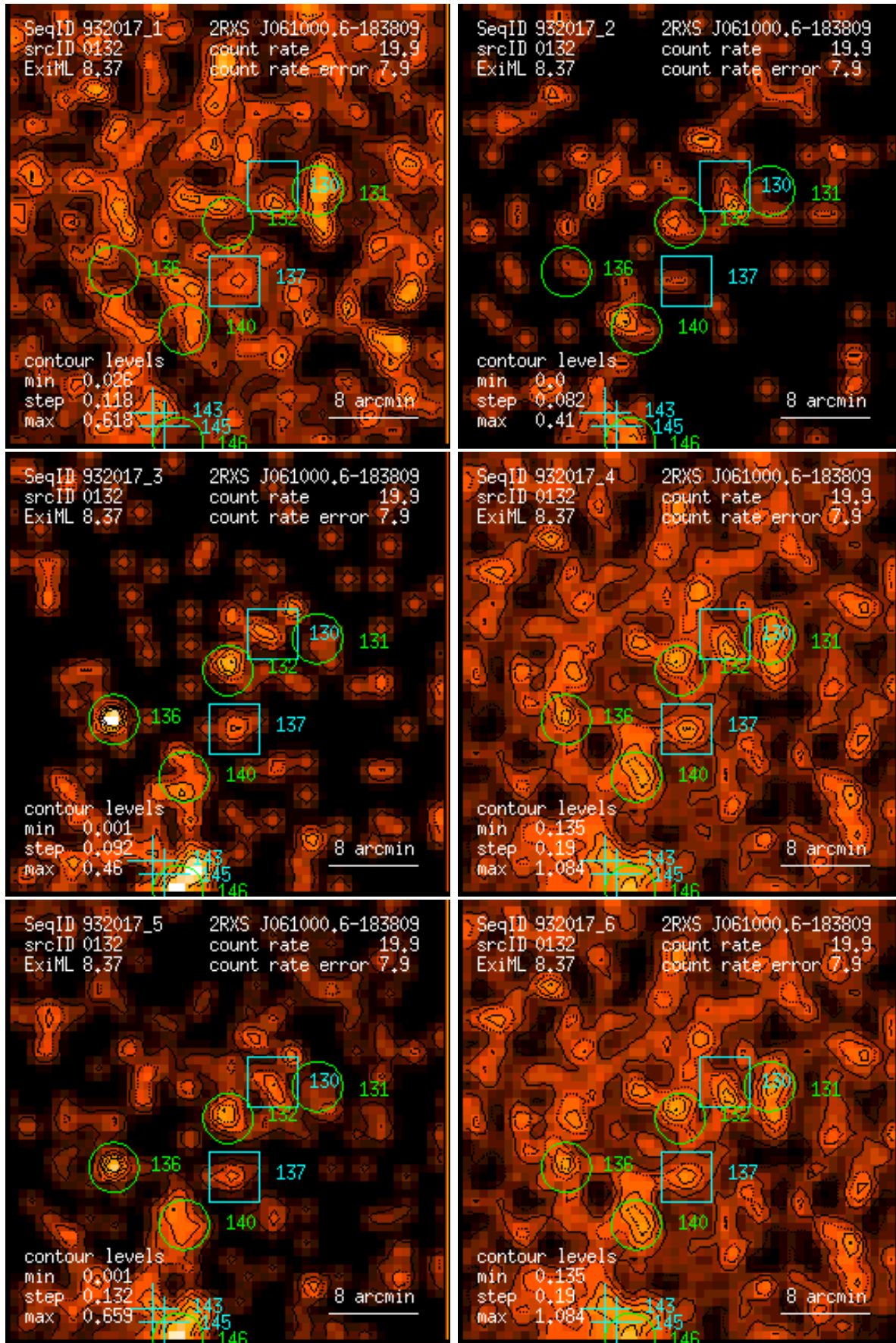
Figure 132: RASS 932017: detection 0132: band rate images, Gaussian filter: (1) PSPC channels 11 – 41, (2) 52 – 90, (3) 91 – 201, (4) 11 – 235, (5) 52 – 201, (6) 11 – 201. Broad band rates in counts/ks. Band rate contour levels in counts/ks/arcmin 2 .
