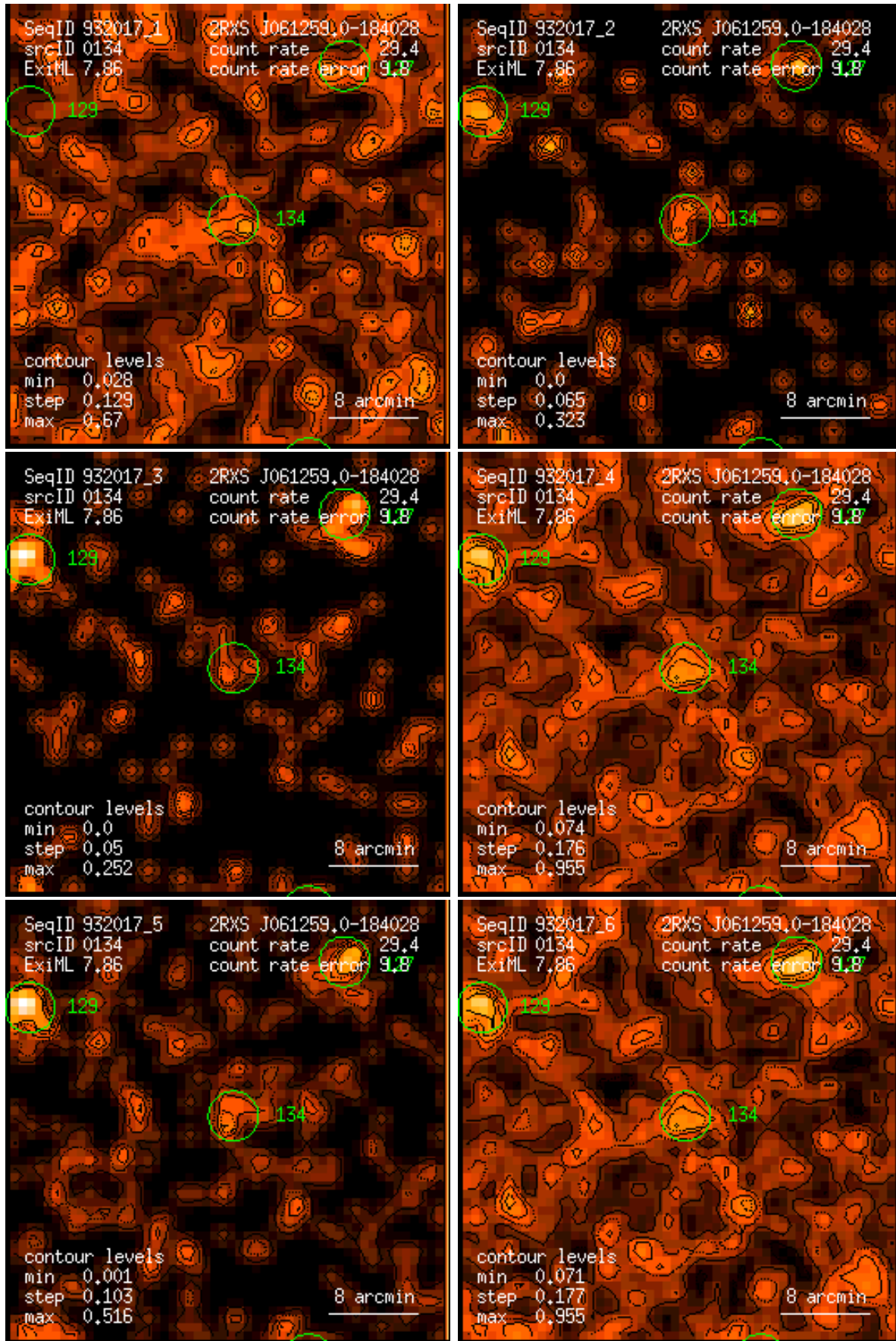
Figure 134: RASS 932017: detection 0134: band rate images, Gaussian filter: (1) PSPC channels 11 – 41, (2) 52 – 90, (3) 91 – 201, (4) 11 – 235, (5) 52 – 201, (6) 11 – 201. Broad band rates in counts/ks. Band rate contour levels in counts/ks/arcmin 2 .
