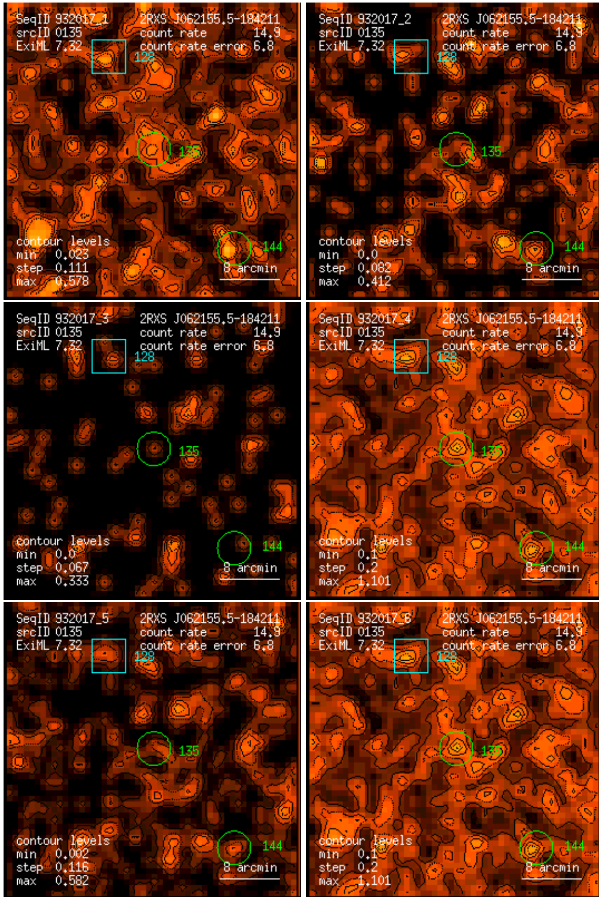
Figure 135: RASS 932017: detection 0135: band rate images, Gaussian filter: (1) PSPC channels 11 – 41, (2) 52 – 90, (3) 91 – 201, (4) 11 – 235, (5) 52 – 201, (6) 11 – 201. Broad band rates in counts/ks. Band rate contour levels in counts/ks/arcmin 2 .
