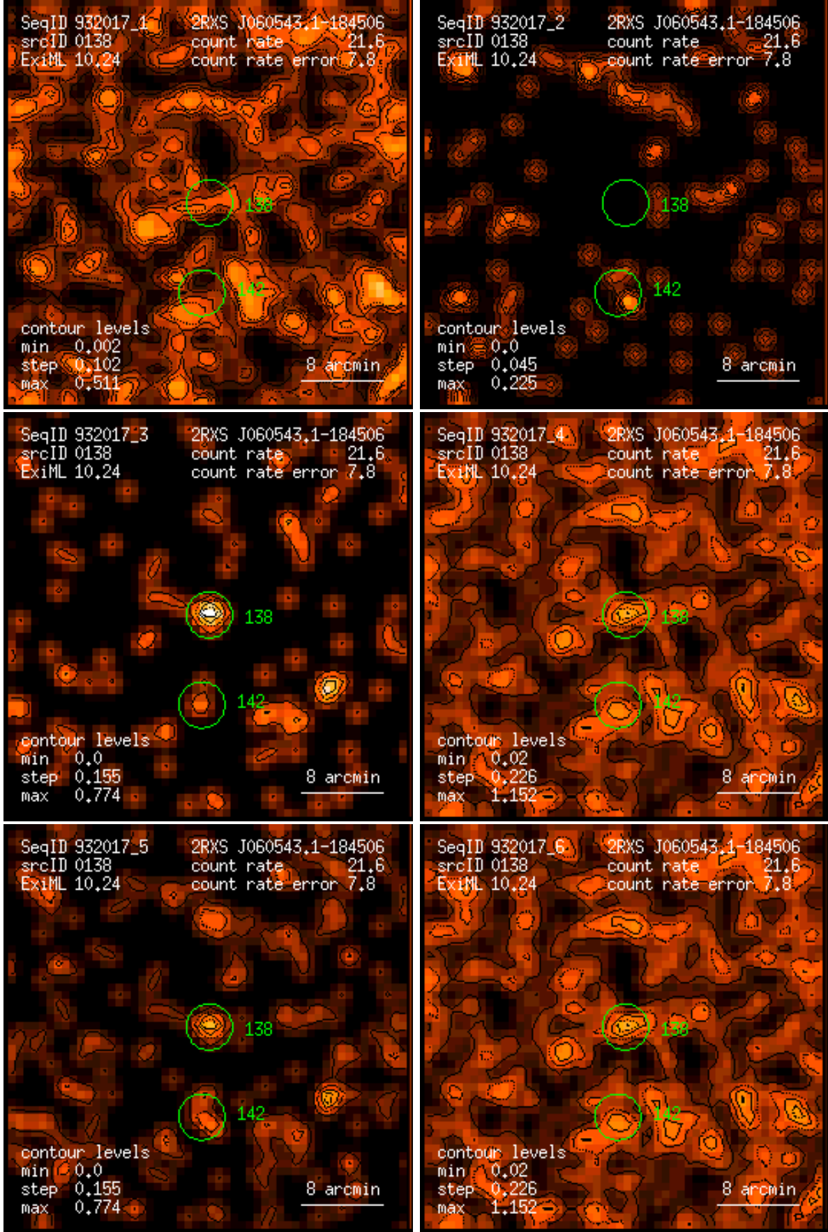
Figure 138: RASS 932017: detection 0138: band rate images, Gaussian filter: (1) PSPC channels 11 – 41, (2) 52 – 90, (3) 91 – 201, (4) 11 – 235, (5) 52 – 201, (6) 11 – 201. Broad band rates in counts/ks. Band rate contour levels in counts/ks/arcmin 2 .
