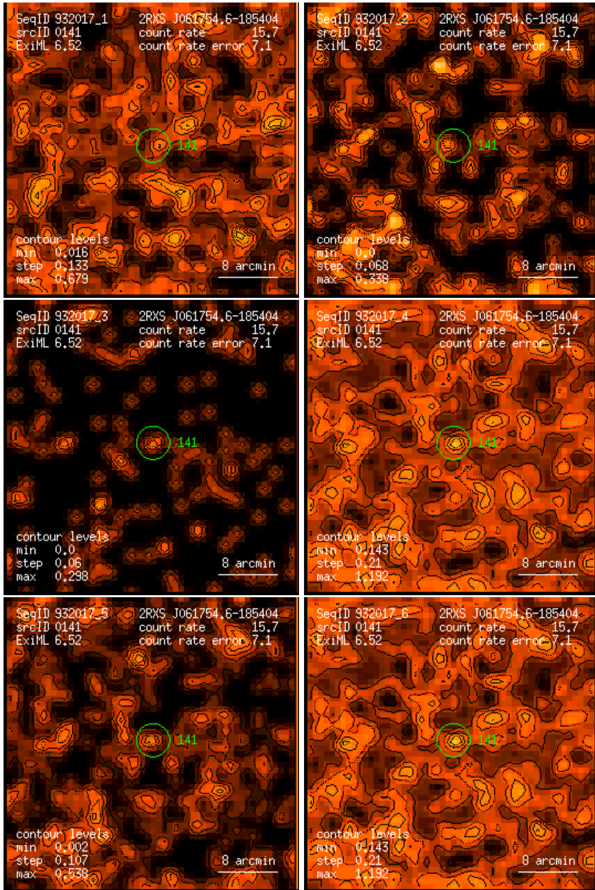
Figure 141: RASS 932017: detection 0141: band rate images, Gaussian filter: (1) PSPC channels 11 – 41, (2) 52 – 90, (3) 91 – 201, (4) 11 – 235, (5) 52 – 201, (6) 11 – 201. Broad band rates in counts/ks. Band rate contour levels in counts/ks/arcmin 2 .
