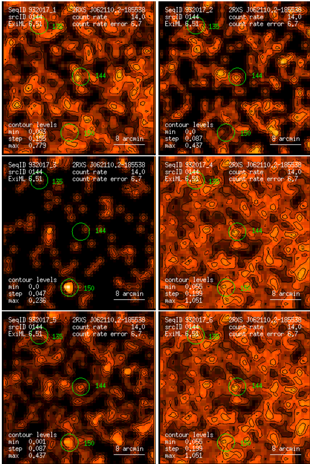
Figure 144: RASS 932017: detection 0144: band rate images, Gaussian filter: (1) PSPC channels 11 – 41, (2) 52 – 90, (3) 91 – 201, (4) 11 – 235, (5) 52 – 201, (6) 11 – 201. Broad band rates in counts/ks. Band rate contour levels in counts/ks/arcmin 2 .
