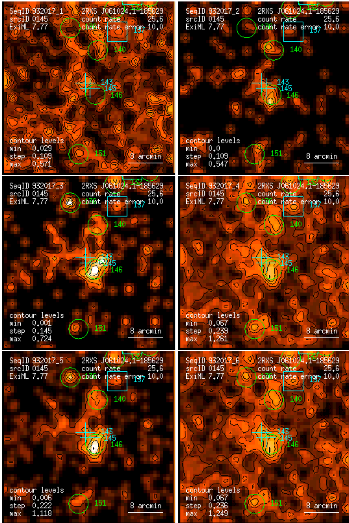
Figure 145: RASS 932017: detection 0145: band rate images, Gaussian filter: (1) PSPC channels 11 – 41, (2) 52 – 90, (3) 91 – 201, (4) 11 – 235, (5) 52 – 201, (6) 11 – 201. Broad band rates in counts/ks. Band rate contour levels in counts/ks/arcmin 2 .
