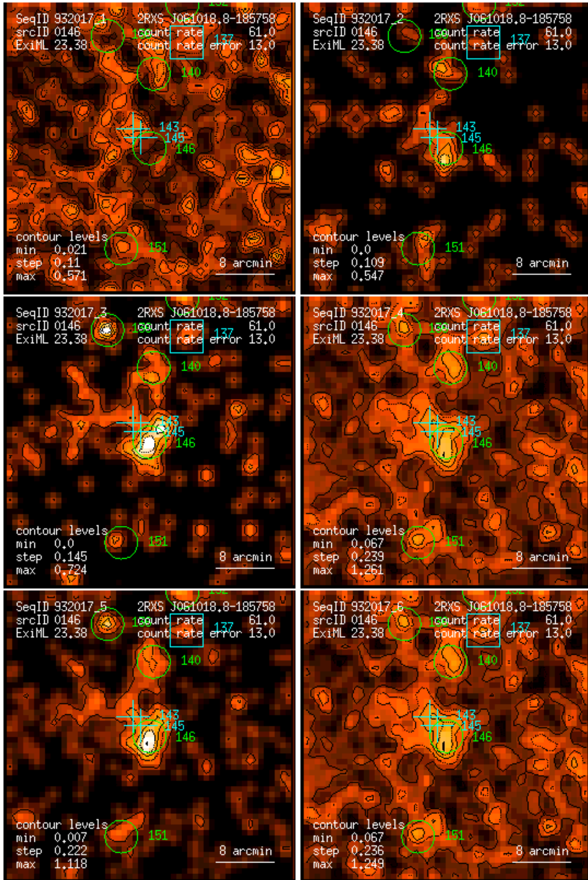
Figure 146: RASS 932017: detection 0146: band rate images, Gaussian filter: (1) PSPC channels 11 – 41, (2) 52 – 90, (3) 91 – 201, (4) 11 – 235, (5) 52 – 201, (6) 11 – 201. Broad band rates in counts/ks. Band rate contour levels in counts/ks/arcmin 2 .
