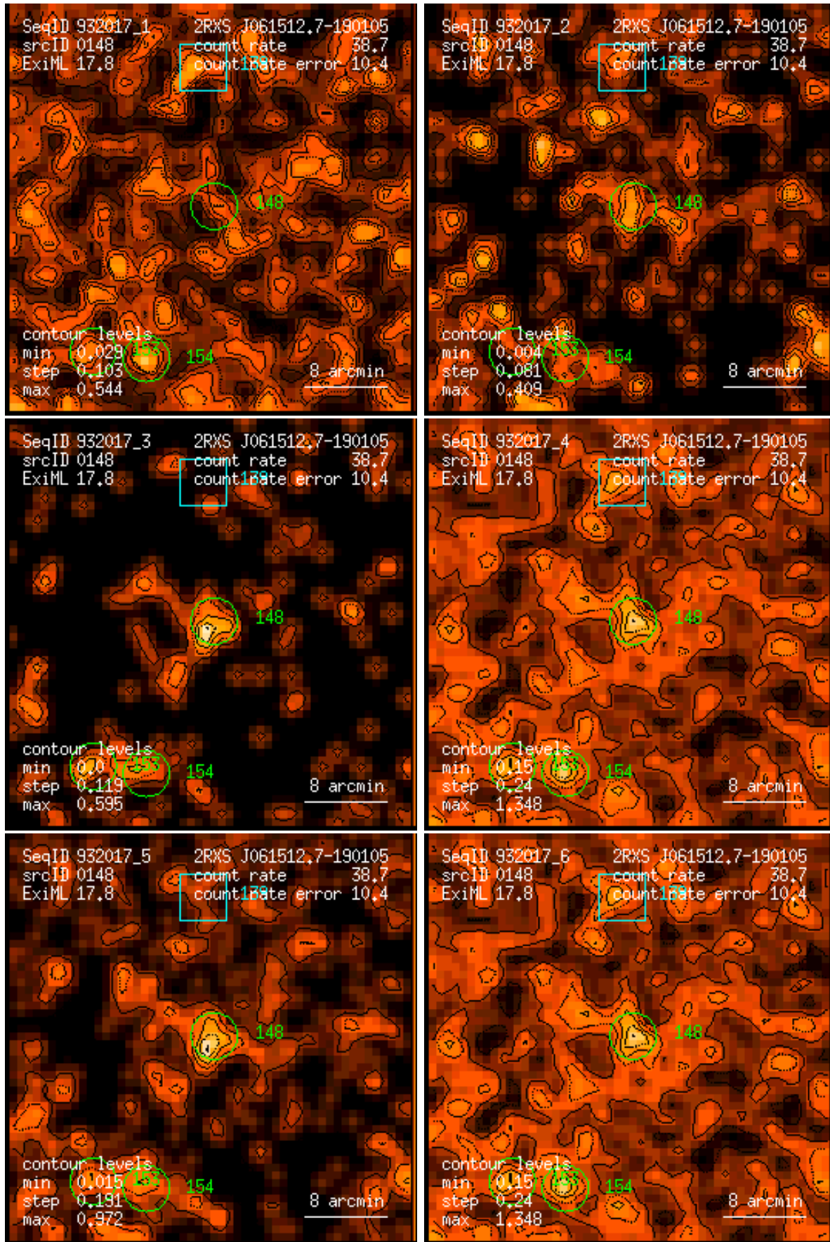
Figure 148: RASS 932017: detection 0148: band rate images, Gaussian filter: (1) PSPC channels 11 – 41, (2) 52 – 90, (3) 91 – 201, (4) 11 – 235, (5) 52 – 201, (6) 11 – 201. Broad band rates in counts/ks. Band rate contour levels in counts/ks/arcmin 2 .
