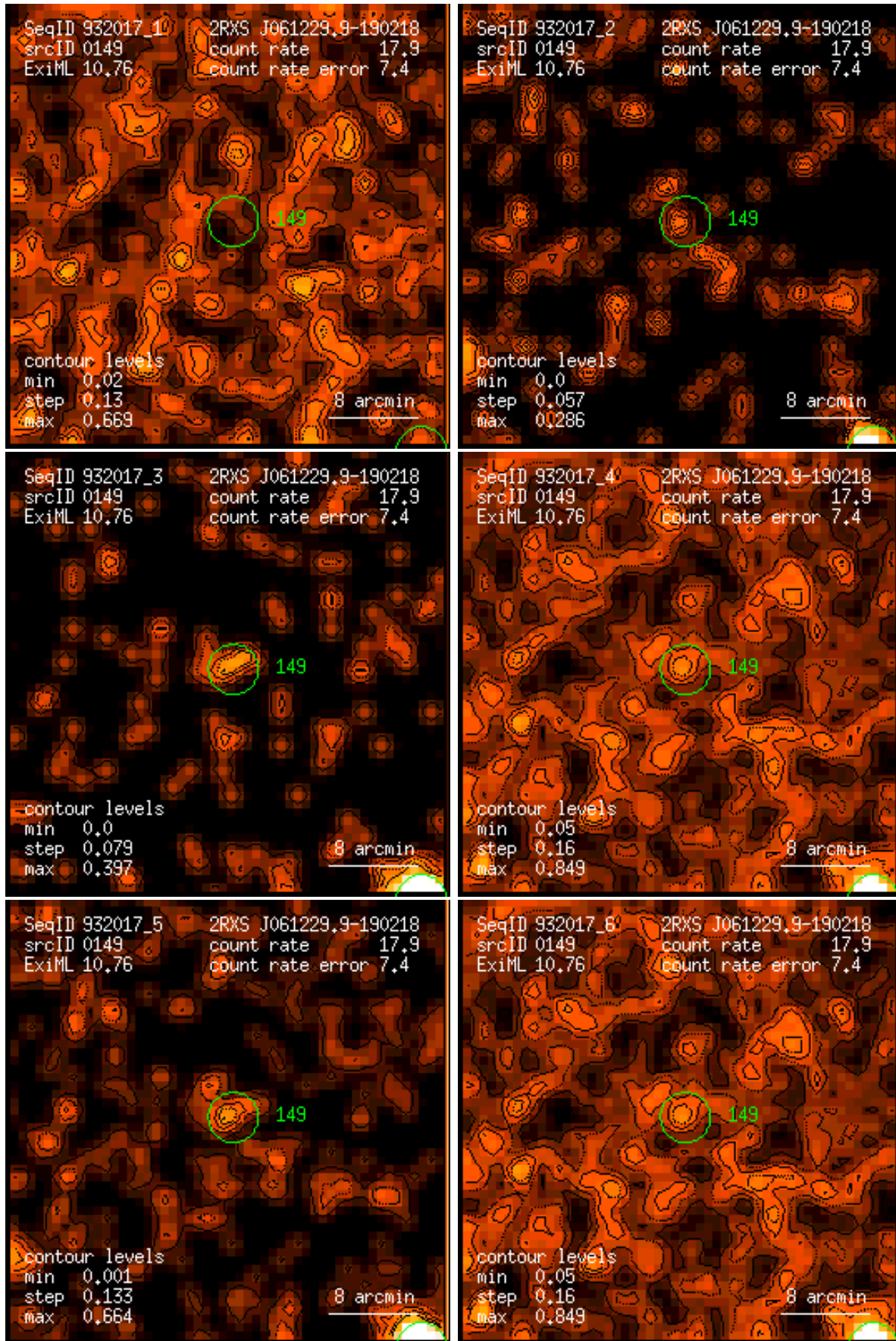
Figure 149: RASS 932017: detection 0149: band rate images, Gaussian filter: (1) PSPC channels 11 – 41, (2) 52 – 90, (3) 91 – 201, (4) 11 – 235, (5) 52 – 201, (6) 11 – 201. Broad band rates in counts/ks. Band rate contour levels in counts/ks/arcmin 2 .
