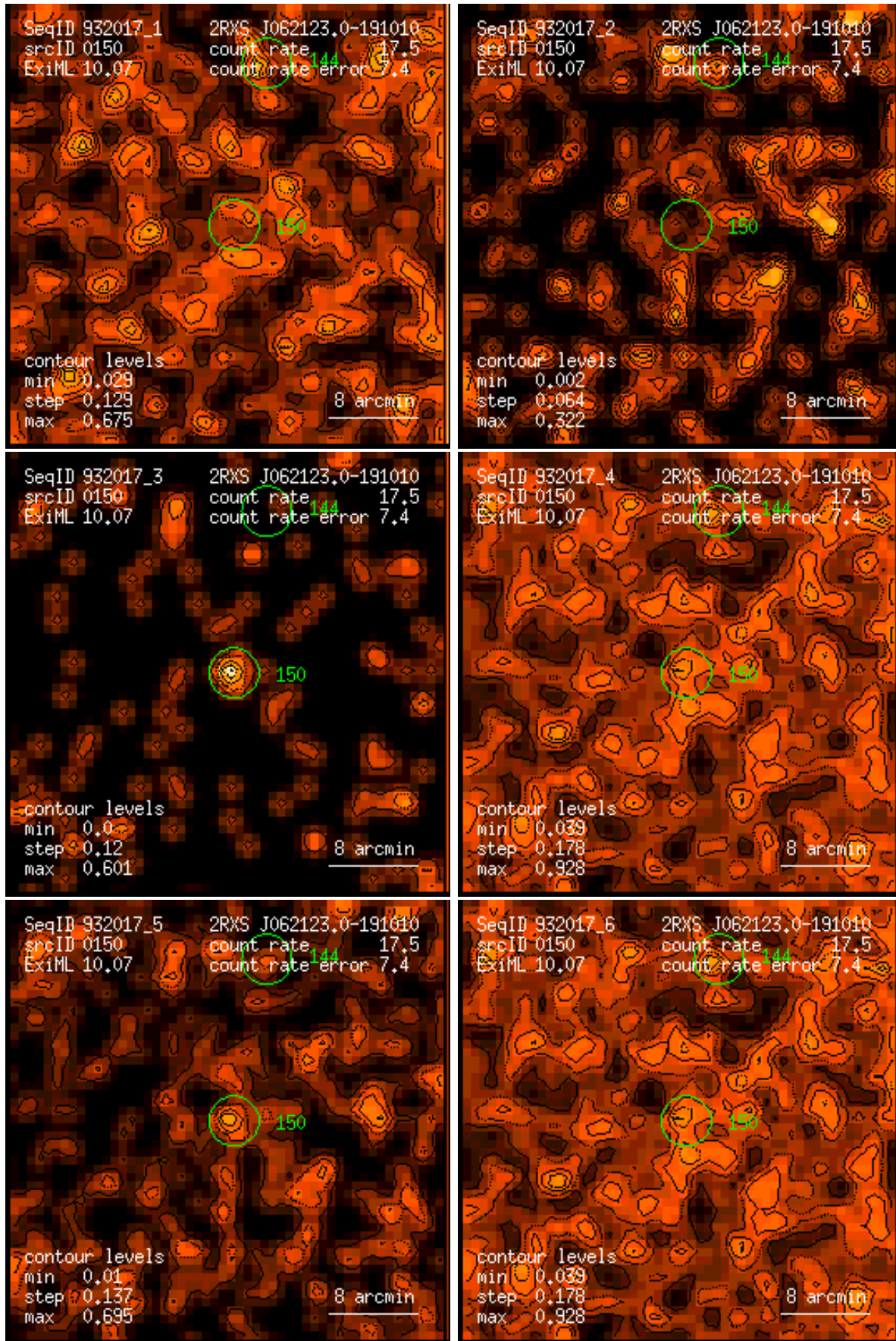
Figure 150: RASS 932017: detection 0150: band rate images, Gaussian filter: (1) PSPC channels 11 – 41, (2) 52 – 90, (3) 91 – 201, (4) 11 – 235, (5) 52 – 201, (6) 11 – 201. Broad band rates in counts/ks. Band rate contour levels in counts/ks/arcmin 2 .
