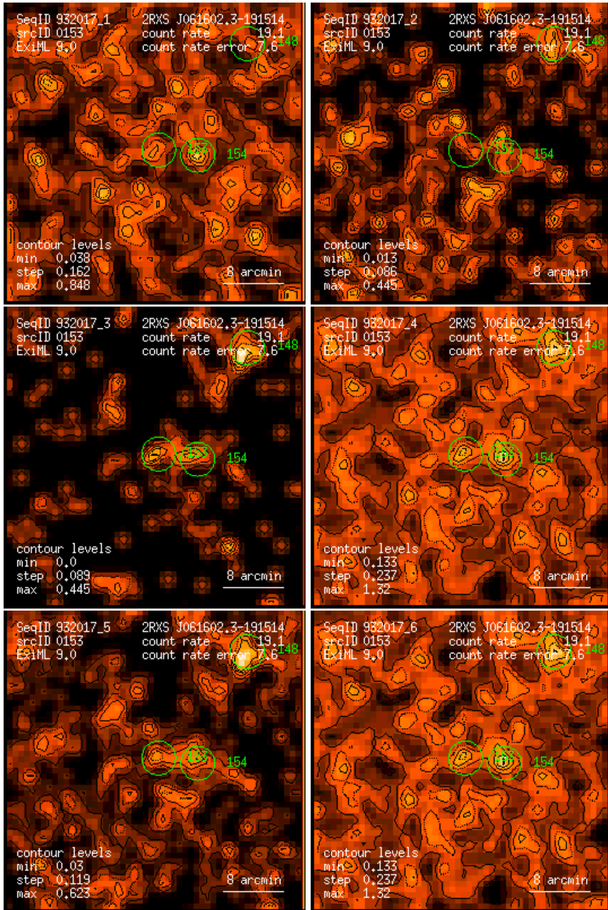
Figure 153: RASS 932017: detection 0153: band rate images, Gaussian filter: (1) PSPC channels 11 – 41, (2) 52 – 90, (3) 91 – 201, (4) 11 – 235, (5) 52 – 201, (6) 11 – 201. Broad band rates in counts/ks. Band rate contour levels in counts/ks/arcmin 2 .
