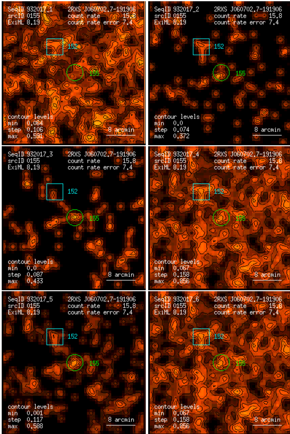
Figure 155: RASS 932017: detection 0155: band rate images, Gaussian filter: (1) PSPC channels 11 – 41, (2) 52 – 90, (3) 91 – 201, (4) 11 – 235, (5) 52 – 201, (6) 11 – 201. Broad band rates in counts/ks. Band rate contour levels in counts/ks/arcmin 2 .
