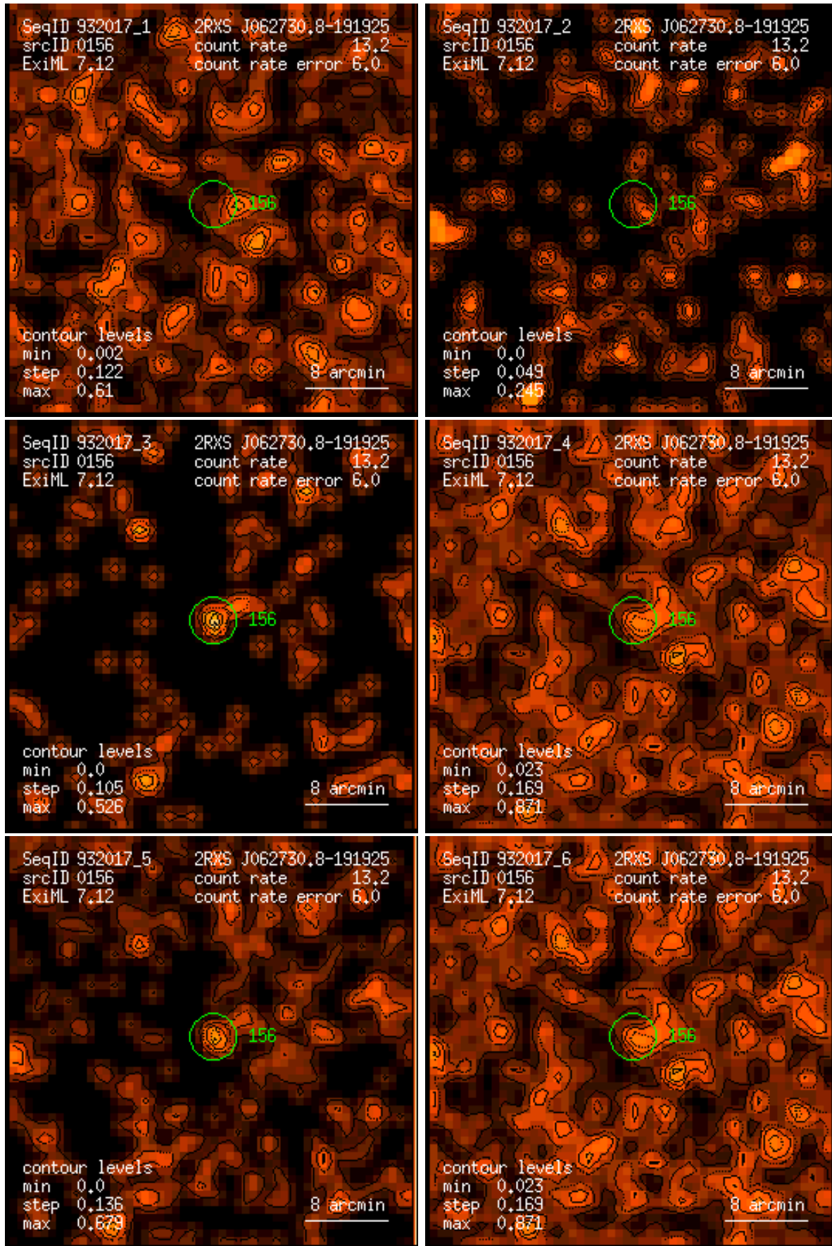
Figure 156: RASS 932017: detection 0156: band rate images, Gaussian filter: (1) PSPC channels 11 – 41, (2) 52 – 90, (3) 91 – 201, (4) 11 – 235, (5) 52 – 201, (6) 11 – 201. Broad band rates in counts/ks. Band rate contour levels in counts/ks/arcmin 2 .
