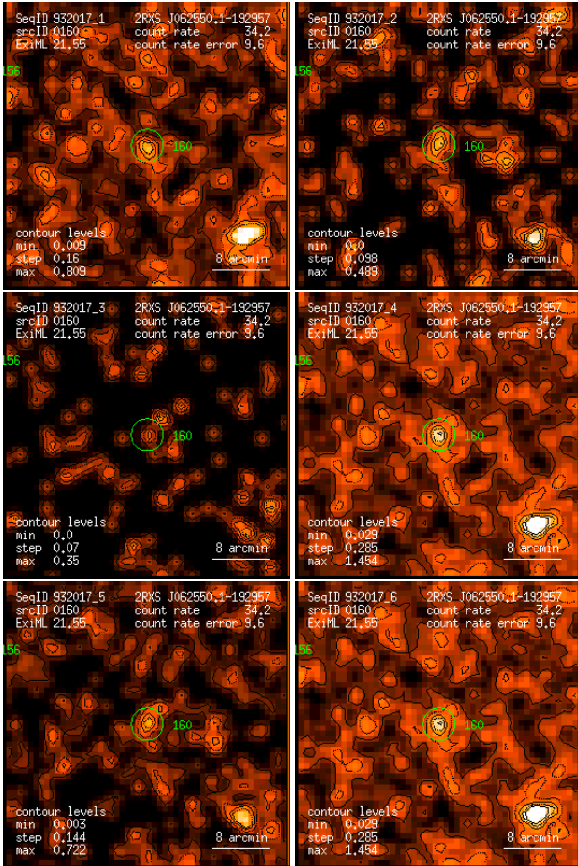
Figure 160: RASS 932017: detection 0160: band rate images, Gaussian filter: (1) PSPC channels 11 – 41, (2) 52 – 90, (3) 91 – 201, (4) 11 – 235, (5) 52 – 201, (6) 11 – 201. Broad band rates in counts/ks. Band rate contour levels in counts/ks/arcmin 2 .
