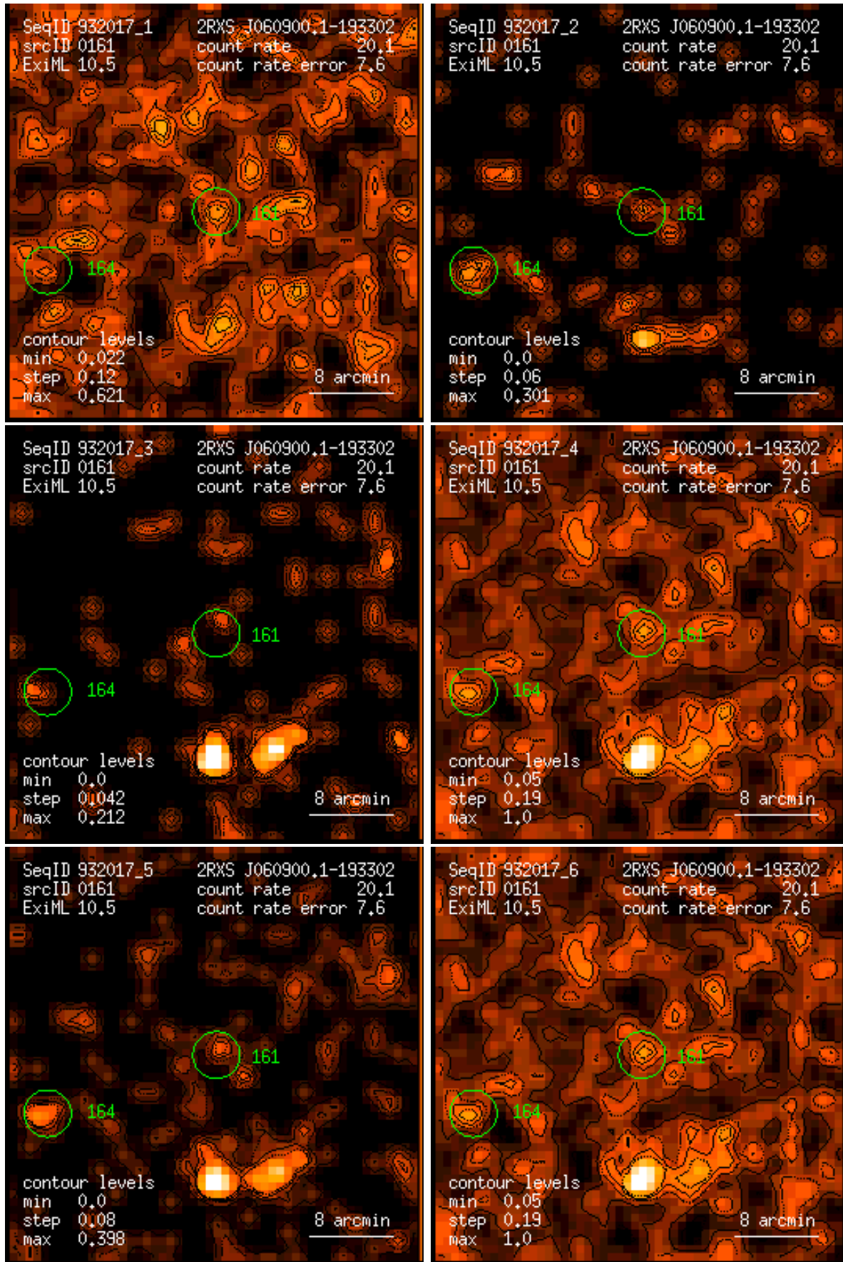
Figure 161: RASS 932017: detection 0161: band rate images, Gaussian filter: (1) PSPC channels 11 – 41, (2) 52 – 90, (3) 91 – 201, (4) 11 – 235, (5) 52 – 201, (6) 11 – 201. Broad band rates in counts/ks. Band rate contour levels in counts/ks/arcmin 2 .
