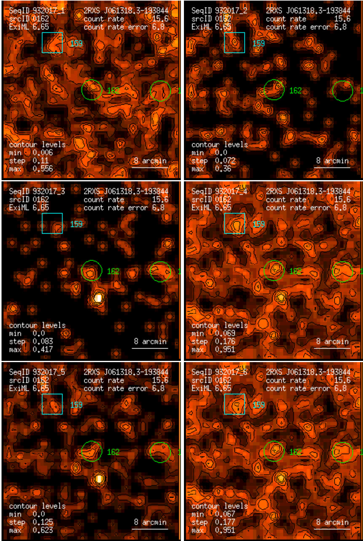
Figure 162: RASS 932017: detection 0162: band rate images, Gaussian filter: (1) PSPC channels 11 – 41, (2) 52 – 90, (3) 91 – 201, (4) 11 – 235, (5) 52 – 201, (6) 11 – 201. Broad band rates in counts/ks. Band rate contour levels in counts/ks/arcmin 2 .
