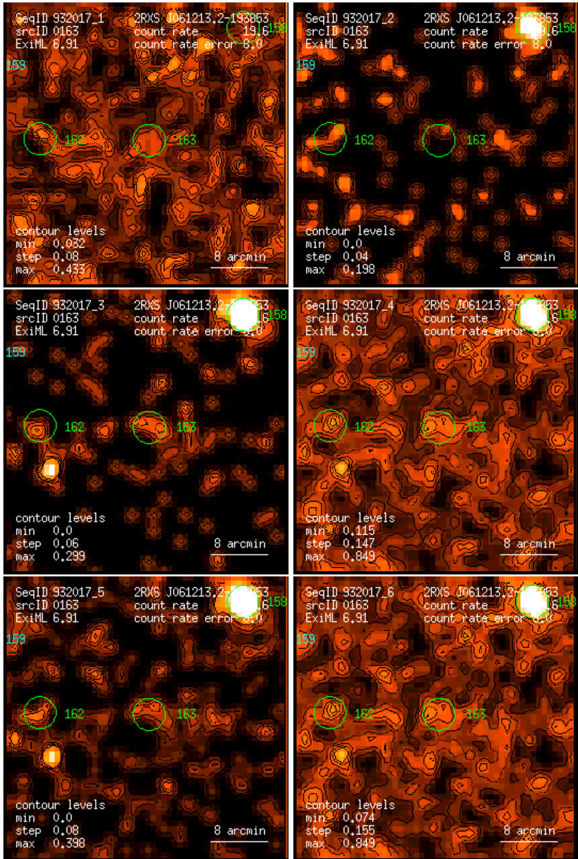
Figure 163: RASS 932017: detection 0163: band rate images, Gaussian filter: (1) PSPC channels 11 – 41, (2) 52 – 90, (3) 91 – 201, (4) 11 – 235, (5) 52 – 201, (6) 11 – 201. Broad band rates in counts/ks. Band rate contour levels in counts/ks/arcmin 2 .
