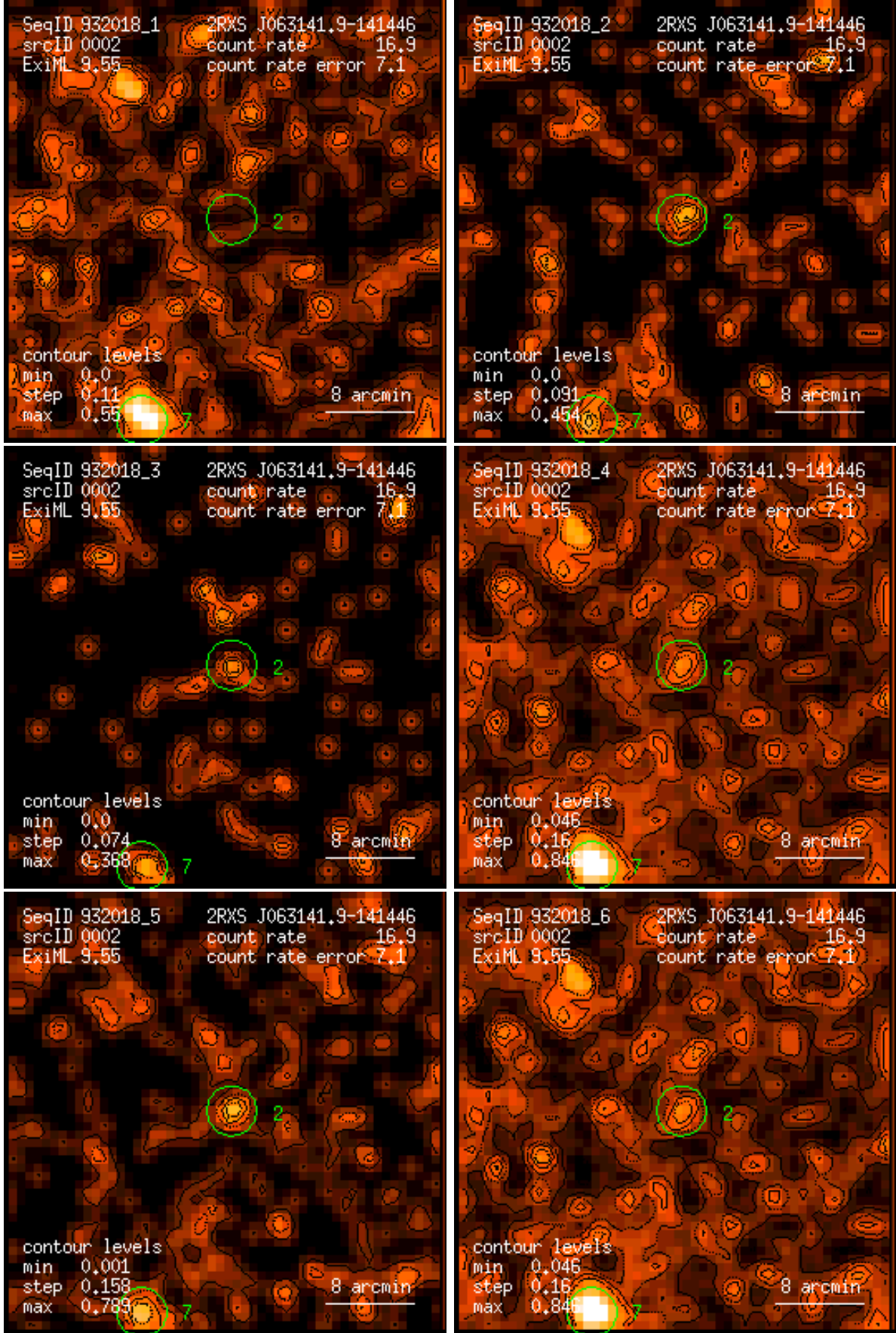
Figure 2: RASS 932018: detection 0002: band rate images, Gaussian filter: (1) PSPC channels 11 – 41, (2) 52 – 90, (3) 91 – 201, (4) 11 – 235, (5) 52 – 201, (6) 11 – 201. Broad band rates in counts/ks. Band rate contour levels in counts/ks/arcmin 2 .
