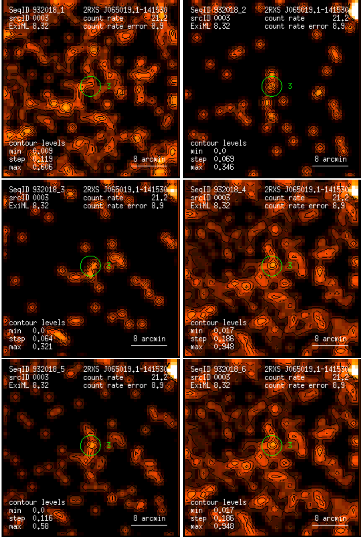
Figure 3: RASS 932018: detection 0003: band rate images, Gaussian filter: (1) PSPC channels 11 – 41, (2) 52 – 90, (3) 91 – 201, (4) 11 – 235, (5) 52 – 201, (6) 11 – 201. Broad band rates in counts/ks. Band rate contour levels in counts/ks/arcmin 2 .
