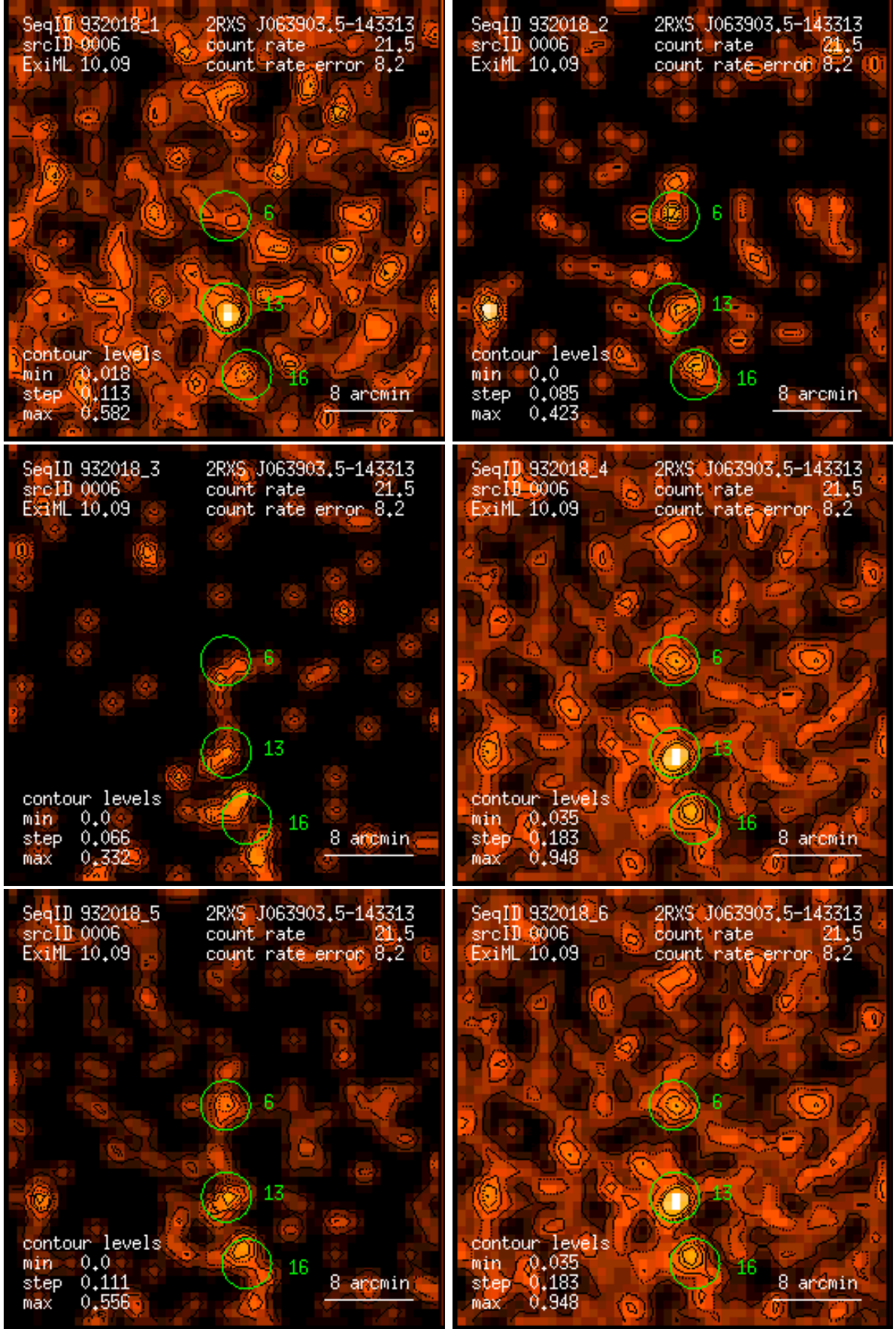
Figure 6: RASS 932018: detection 0006: band rate images, Gaussian filter: (1) PSPC channels 11 – 41, (2) 52 – 90, (3) 91 – 201, (4) 11 – 235, (5) 52 – 201, (6) 11 – 201. Broad band rates in counts/ks. Band rate contour levels in counts/ks/arcmin 2 .
