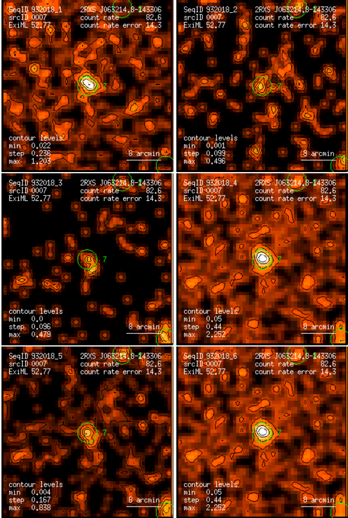
Figure 7: RASS 932018: detection 0007: band rate images, Gaussian filter: (1) PSPC channels 11 – 41, (2) 52 – 90, (3) 91 – 201, (4) 11 – 235, (5) 52 – 201, (6) 11 – 201. Broad band rates in counts/ks. Band rate contour levels in counts/ks/arcmin 2 .
