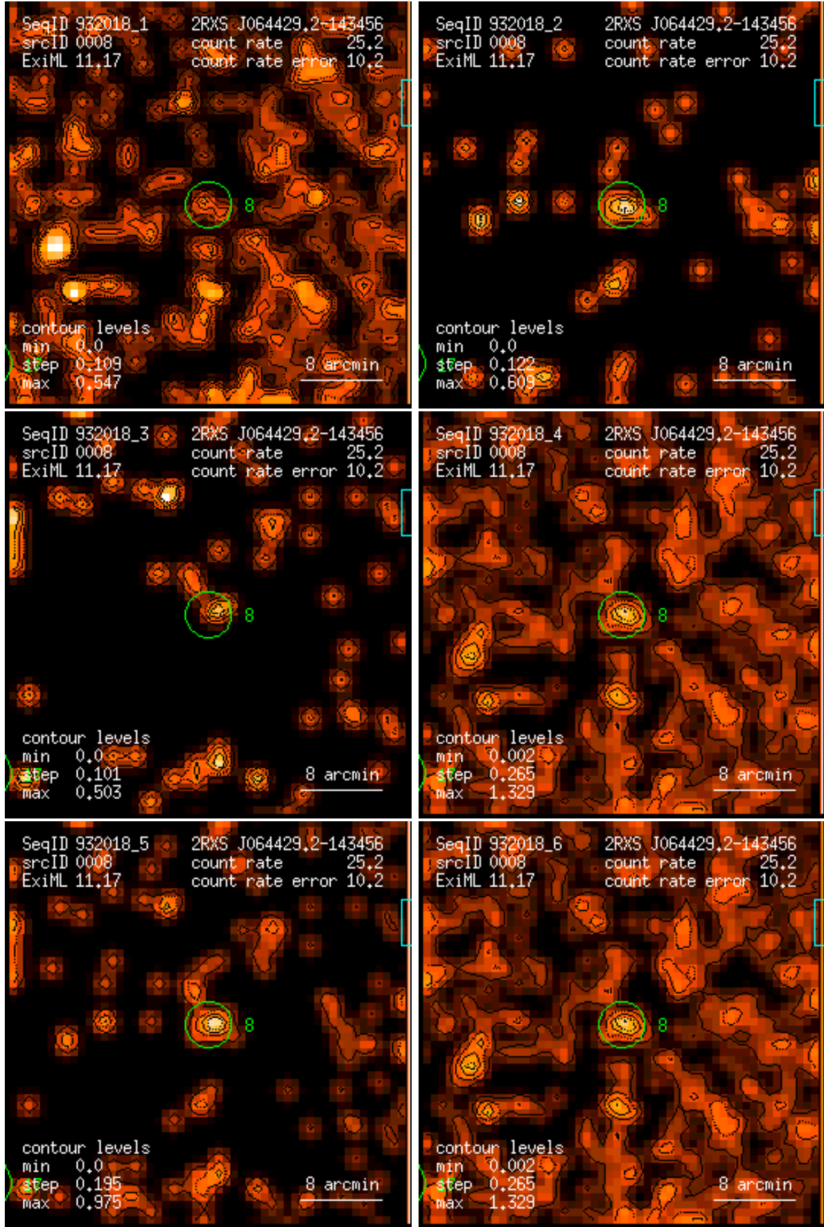
Figure 8: RASS 932018: detection 0008: band rate images, Gaussian filter: (1) PSPC channels 11 – 41, (2) 52 – 90, (3) 91 – 201, (4) 11 – 235, (5) 52 – 201, (6) 11 – 201. Broad band rates in counts/ks. Band rate contour levels in counts/ks/arcmin 2 .
