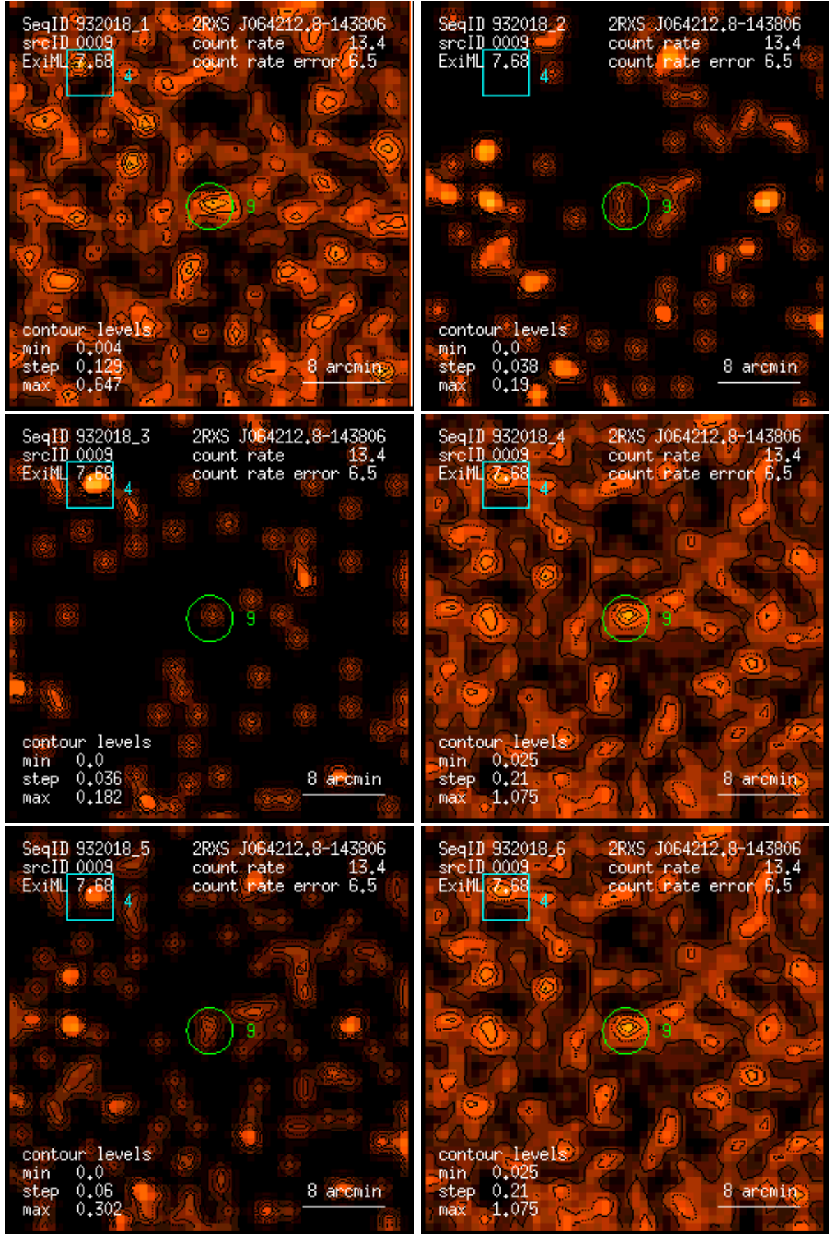
Figure 9: RASS 932018: detection 0009: band rate images, Gaussian filter: (1) PSPC channels 11 – 41, (2) 52 – 90, (3) 91 – 201, (4) 11 – 235, (5) 52 – 201, (6) 11 – 201. Broad band rates in counts/ks. Band rate contour levels in counts/ks/arcmin 2 .
