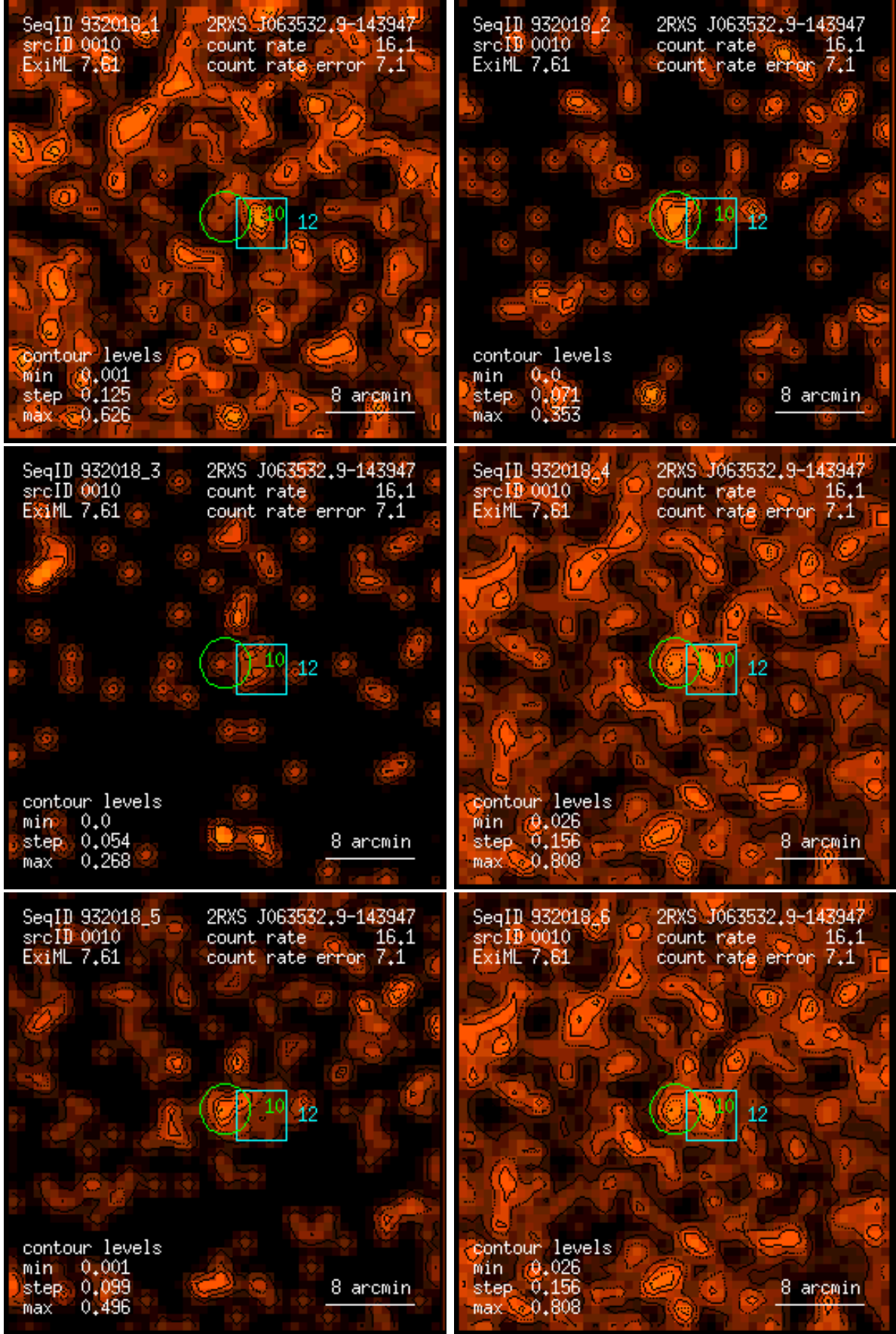
Figure 10: RASS 932018: detection 0010: band rate images, Gaussian filter: (1) PSPC channels 11 – 41, (2) 52 – 90, (3) 91 – 201, (4) 11 – 235, (5) 52 – 201, (6) 11 – 201. Broad band rates in counts/ks. Band rate contour levels in counts/ks/arcmin 2 .
