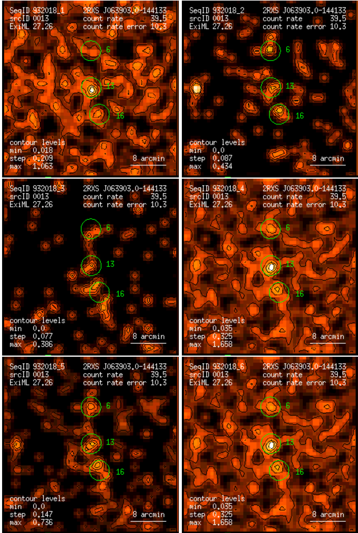
Figure 13: RASS 932018: detection 0013: band rate images, Gaussian filter: (1) PSPC channels 11 – 41, (2) 52 – 90, (3) 91 – 201, (4) 11 – 235, (5) 52 – 201, (6) 11 – 201. Broad band rates in counts/ks. Band rate contour levels in counts/ks/arcmin 2 .
