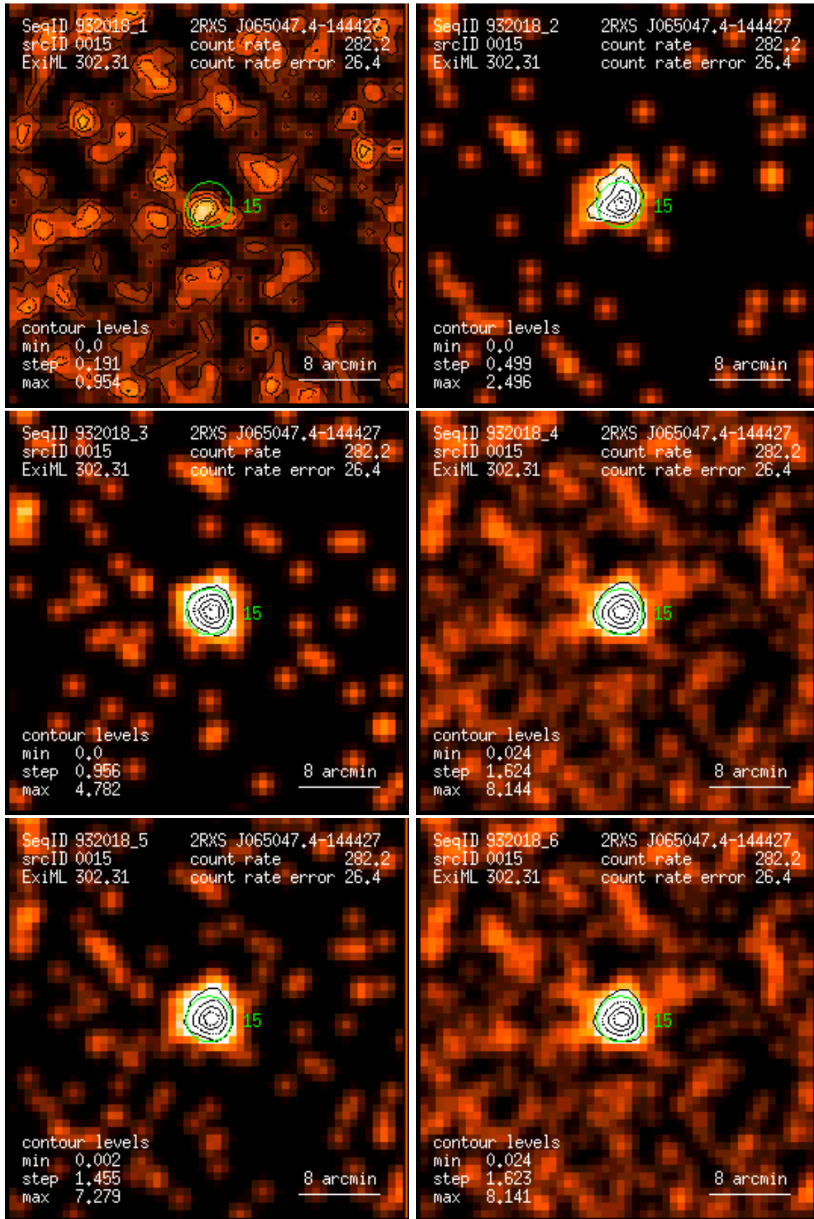
Figure 15: RASS 932018: detection 0015: band rate images, Gaussian filter: (1) PSPC channels 11 – 41, (2) 52 – 90, (3) 91 – 201, (4) 11 – 235, (5) 52 – 201, (6) 11 – 201. Broad band rates in counts/ks. Band rate contour levels in counts/ks/arcmin 2 .
