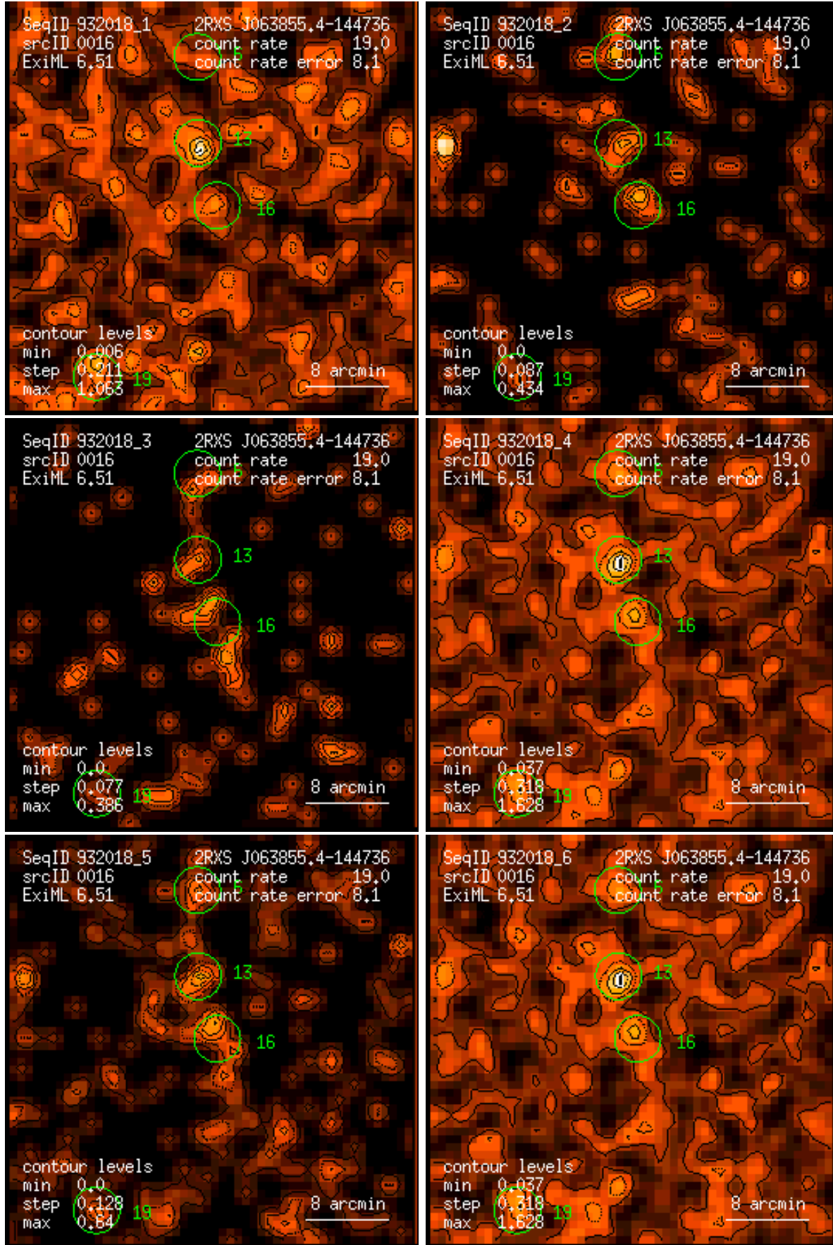
Figure 16: RASS 932018: detection 0016: band rate images, Gaussian filter: (1) PSPC channels 11 – 41, (2) 52 – 90, (3) 91 – 201, (4) 11 – 235, (5) 52 – 201, (6) 11 – 201. Broad band rates in counts/ks. Band rate contour levels in counts/ks/arcmin 2 .
