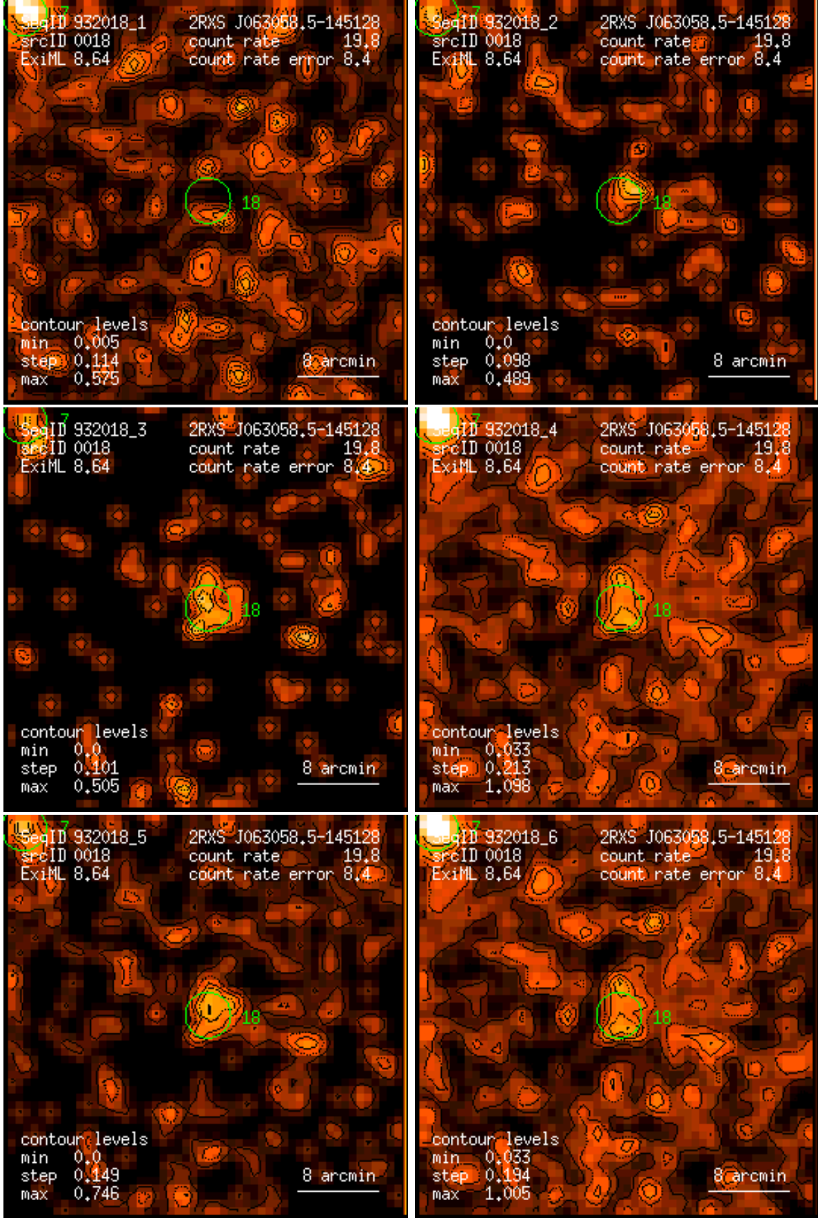
Figure 18: RASS 932018: detection 0018: band rate images, Gaussian filter: (1) PSPC channels 11 – 41, (2) 52 – 90, (3) 91 – 201, (4) 11 – 235, (5) 52 – 201, (6) 11 – 201. Broad band rates in counts/ks. Band rate contour levels in counts/ks/arcmin 2 .
