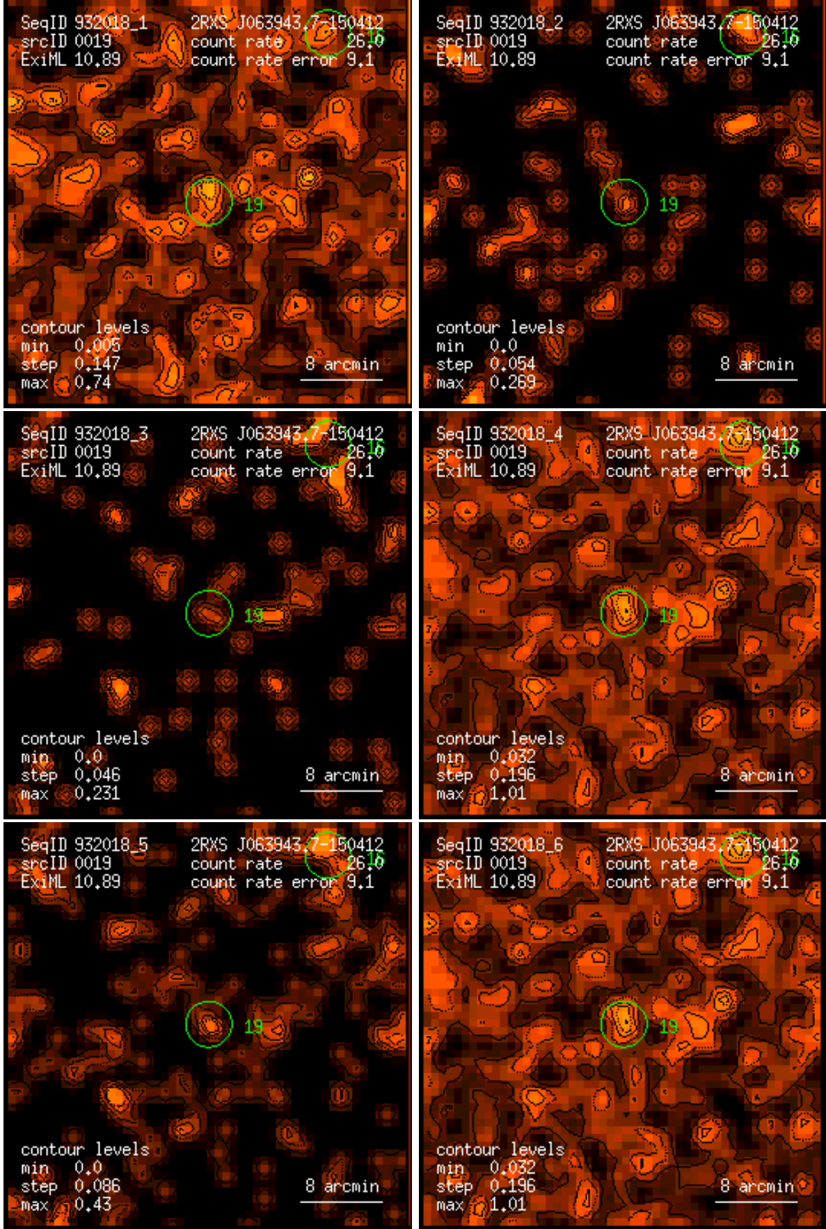
Figure 19: RASS 932018: detection 0019: band rate images, Gaussian filter: (1) PSPC channels 11 – 41, (2) 52 – 90, (3) 91 – 201, (4) 11 – 235, (5) 52 – 201, (6) 11 – 201. Broad band rates in counts/ks. Band rate contour levels in counts/ks/arcmin 2 .
