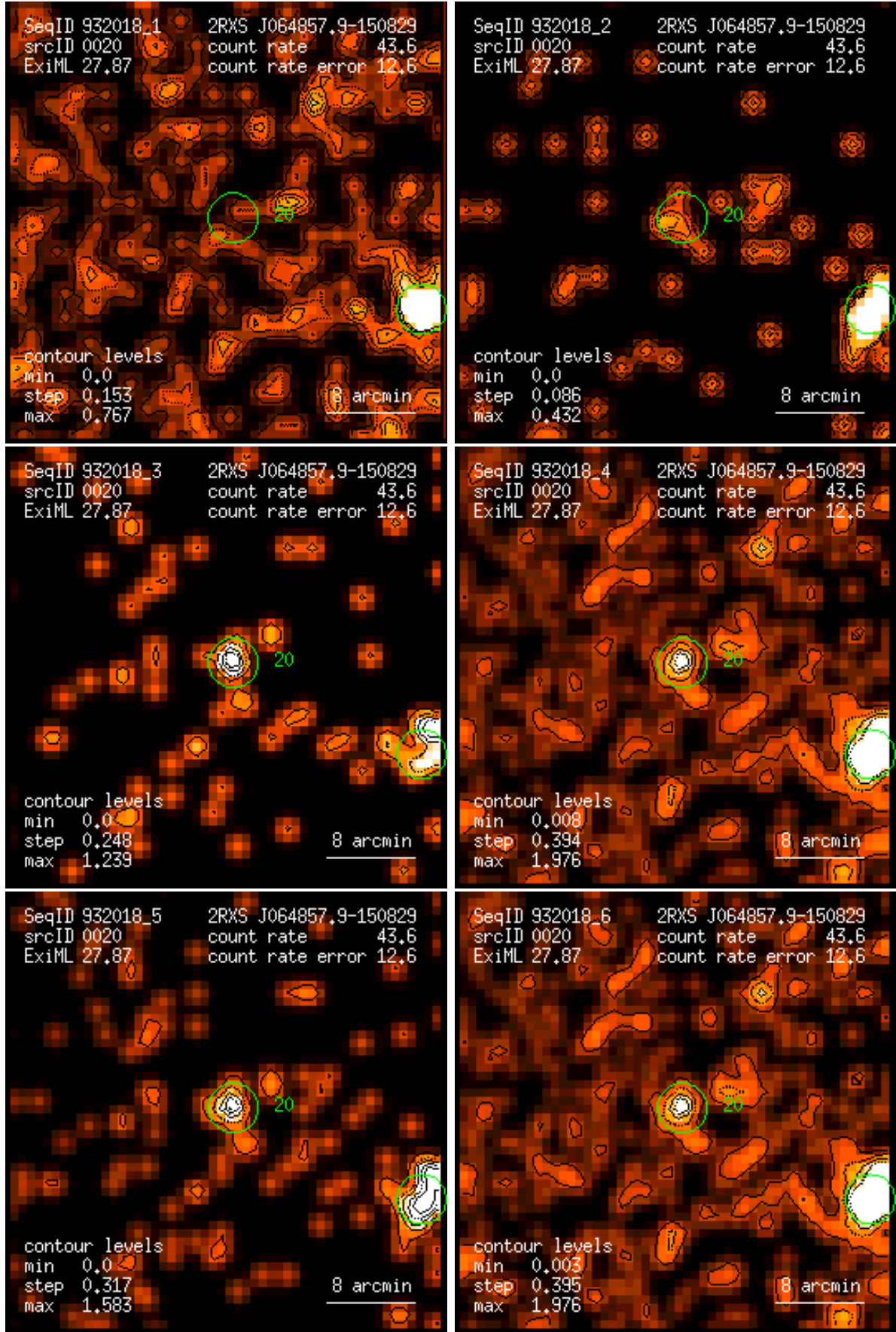
Figure 20: RASS 932018: detection 0020: band rate images, Gaussian filter: (1) PSPC channels 11 – 41, (2) 52 – 90, (3) 91 – 201, (4) 11 – 235, (5) 52 – 201, (6) 11 – 201. Broad band rates in counts/ks. Band rate contour levels in counts/ks/arcmin 2 .
