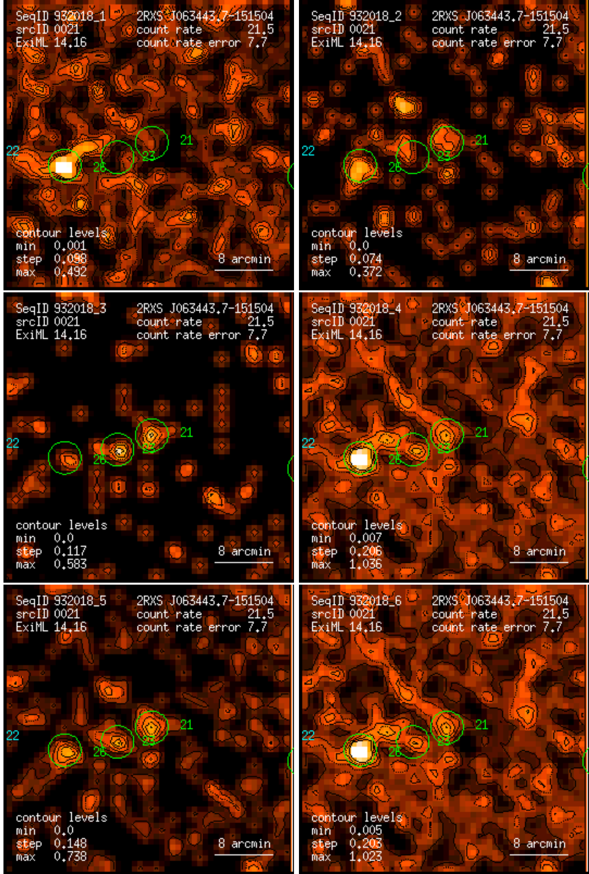
Figure 21: RASS 932018: detection 0021: band rate images, Gaussian filter: (1) PSPC channels 11 – 41, (2) 52 – 90, (3) 91 – 201, (4) 11 – 235, (5) 52 – 201, (6) 11 – 201. Broad band rates in counts/ks. Band rate contour levels in counts/ks/arcmin 2 .
