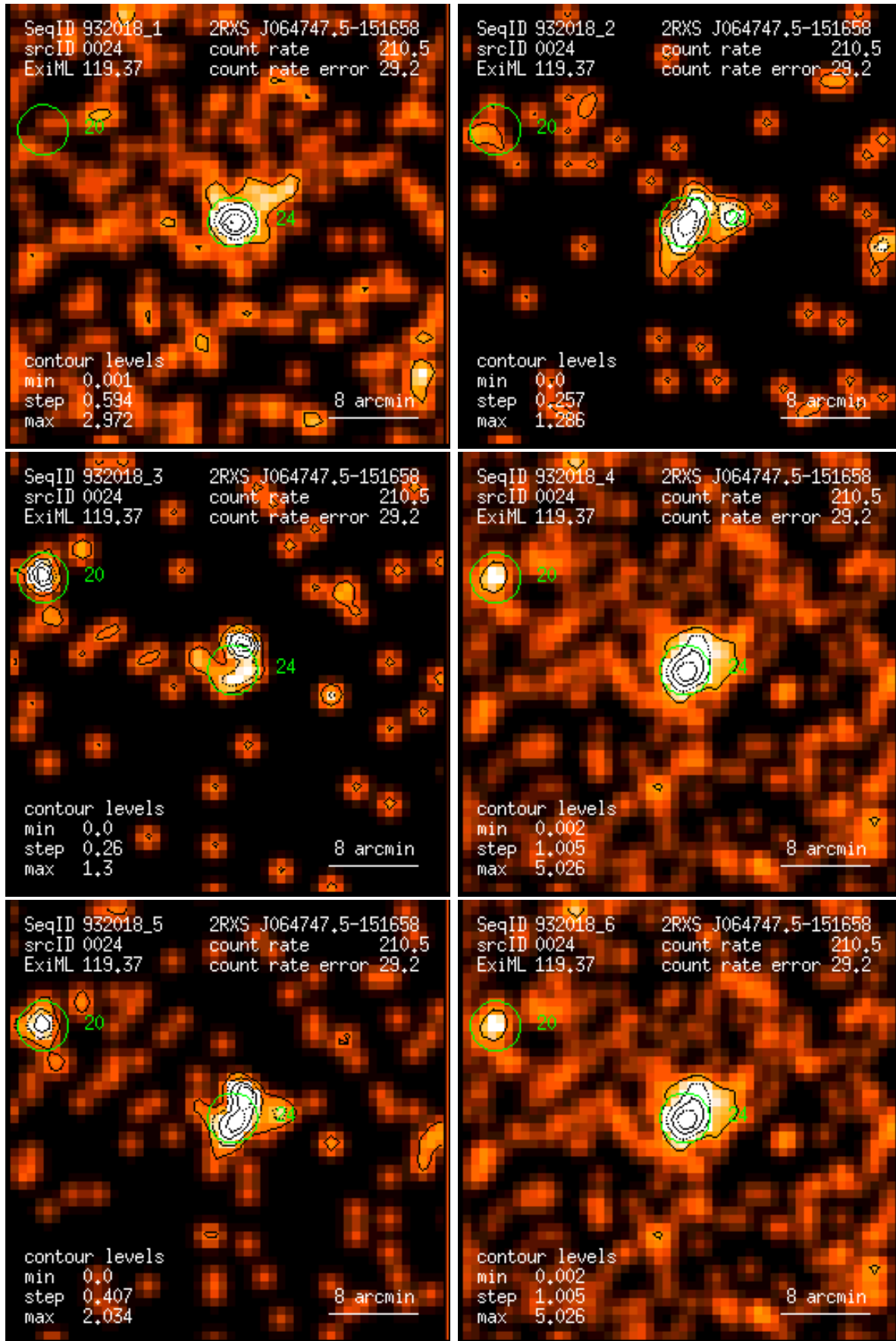
Figure 24: RASS 932018: detection 0024: band rate images, Gaussian filter: (1) PSPC channels 11 – 41, (2) 52 – 90, (3) 91 – 201, (4) 11 – 235, (5) 52 – 201, (6) 11 – 201. Broad band rates in counts/ks. Band rate contour levels in counts/ks/arcmin 2 .
