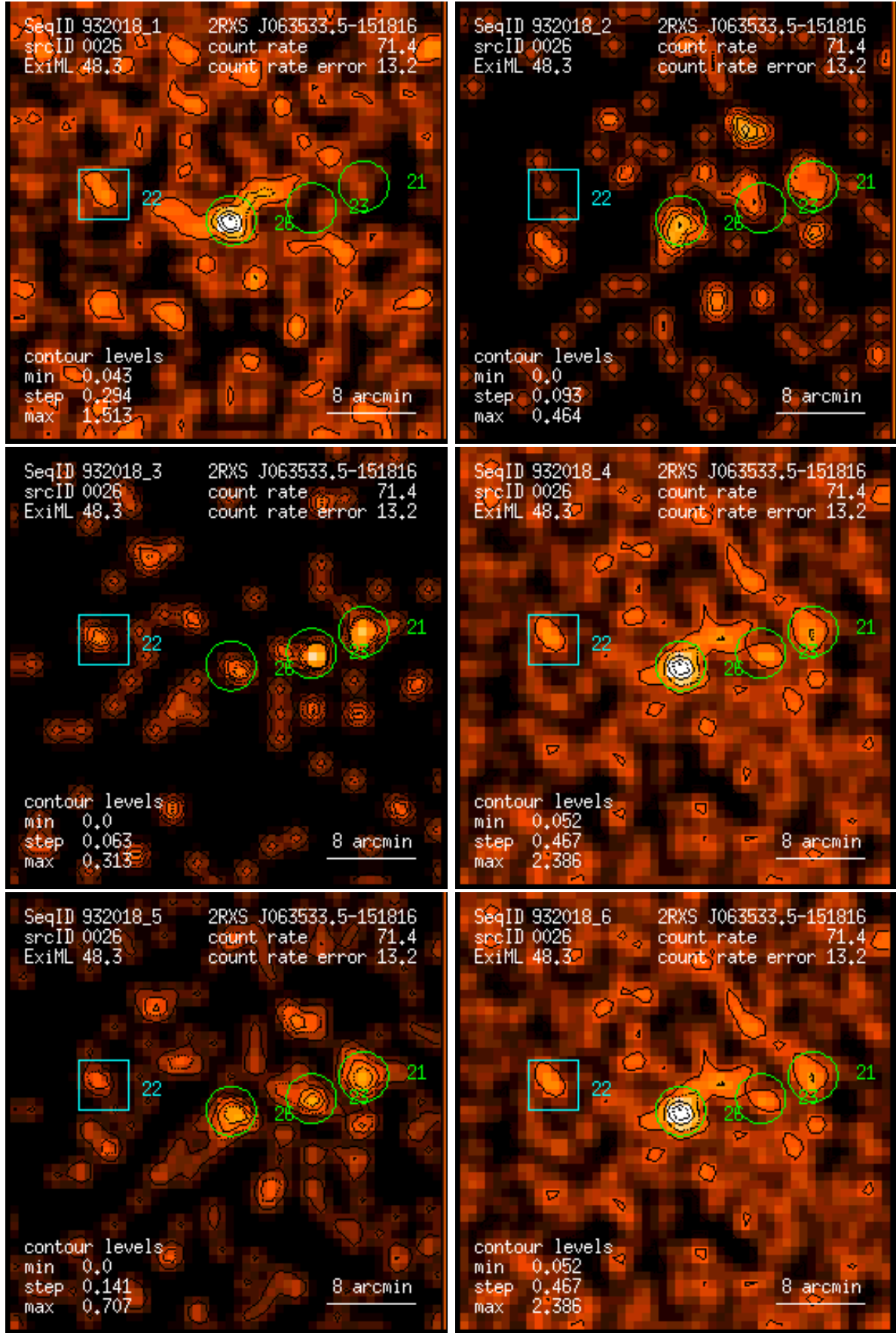
Figure 26: RASS 932018: detection 0026: band rate images, Gaussian filter: (1) PSPC channels 11 – 41, (2) 52 – 90, (3) 91 – 201, (4) 11 – 235, (5) 52 – 201, (6) 11 – 201. Broad band rates in counts/ks. Band rate contour levels in counts/ks/arcmin 2 .
