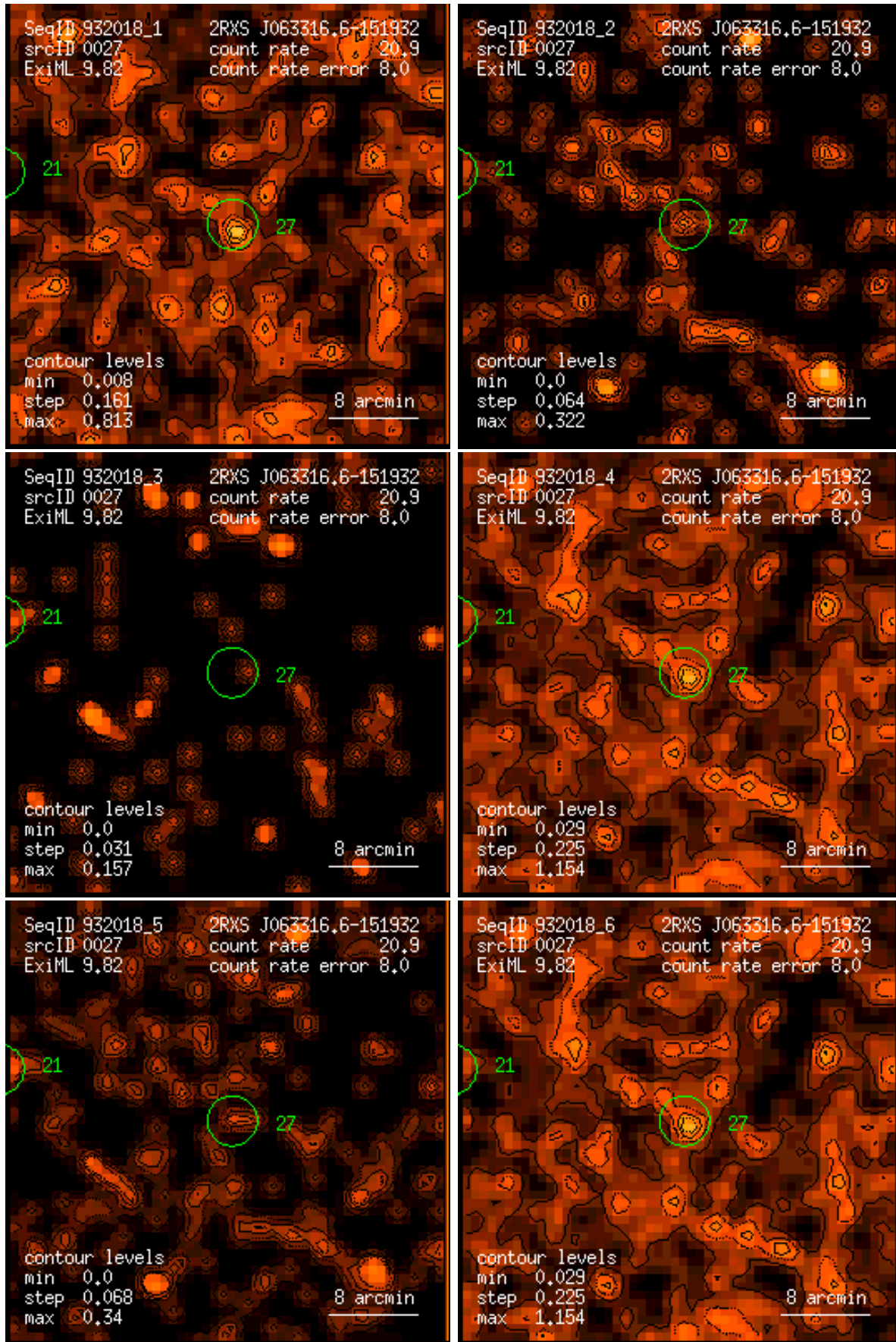
Figure 27: RASS 932018: detection 0027: band rate images, Gaussian filter: (1) PSPC channels 11 – 41, (2) 52 – 90, (3) 91 – 201, (4) 11 – 235, (5) 52 – 201, (6) 11 – 201. Broad band rates in counts/ks. Band rate contour levels in counts/ks/arcmin 2 .
