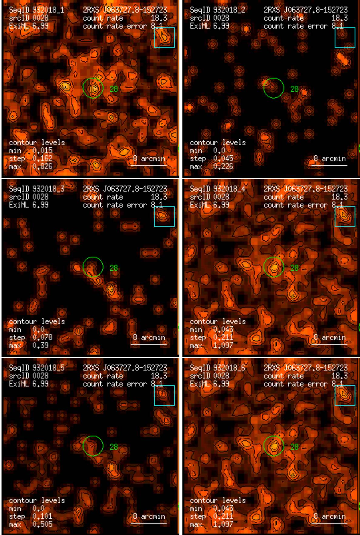
Figure 28: RASS 932018: detection 0028: band rate images, Gaussian filter: (1) PSPC channels 11 – 41, (2) 52 – 90, (3) 91 – 201, (4) 11 – 235, (5) 52 – 201, (6) 11 – 201. Broad band rates in counts/ks. Band rate contour levels in counts/ks/arcmin 2 .
