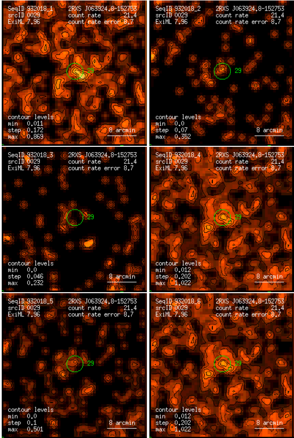
Figure 29: RASS 932018: detection 0029: band rate images, Gaussian filter: (1) PSPC channels 11 – 41, (2) 52 – 90, (3) 91 – 201, (4) 11 – 235, (5) 52 – 201, (6) 11 – 201. Broad band rates in counts/ks. Band rate contour levels in counts/ks/arcmin 2 .
