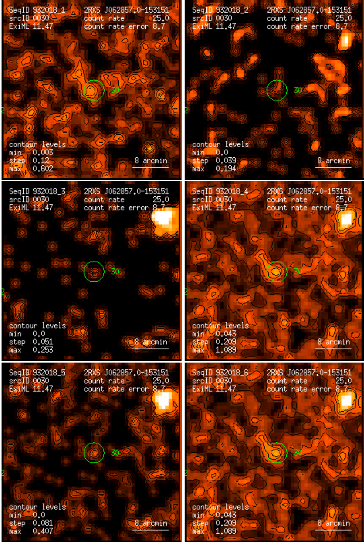
Figure 30: RASS 932018: detection 0030: band rate images, Gaussian filter: (1) PSPC channels 11 – 41, (2) 52 – 90, (3) 91 – 201, (4) 11 – 235, (5) 52 – 201, (6) 11 – 201. Broad band rates in counts/ks. Band rate contour levels in counts/ks/arcmin 2 .
