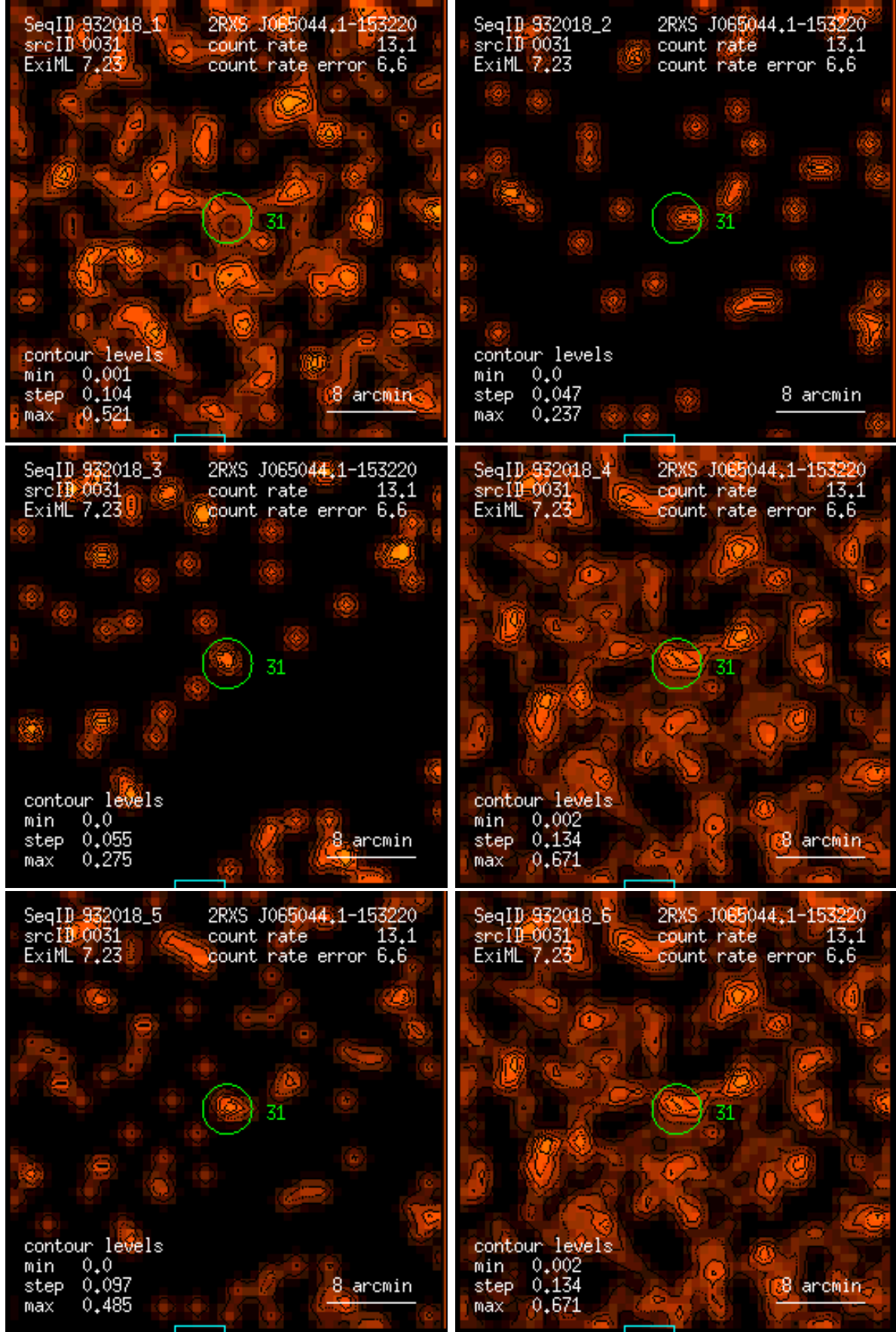
Figure 31: RASS 932018: detection 0031: band rate images, Gaussian filter: (1) PSPC channels 11 – 41, (2) 52 – 90, (3) 91 – 201, (4) 11 – 235, (5) 52 – 201, (6) 11 – 201. Broad band rates in counts/ks. Band rate contour levels in counts/ks/arcmin 2 .
