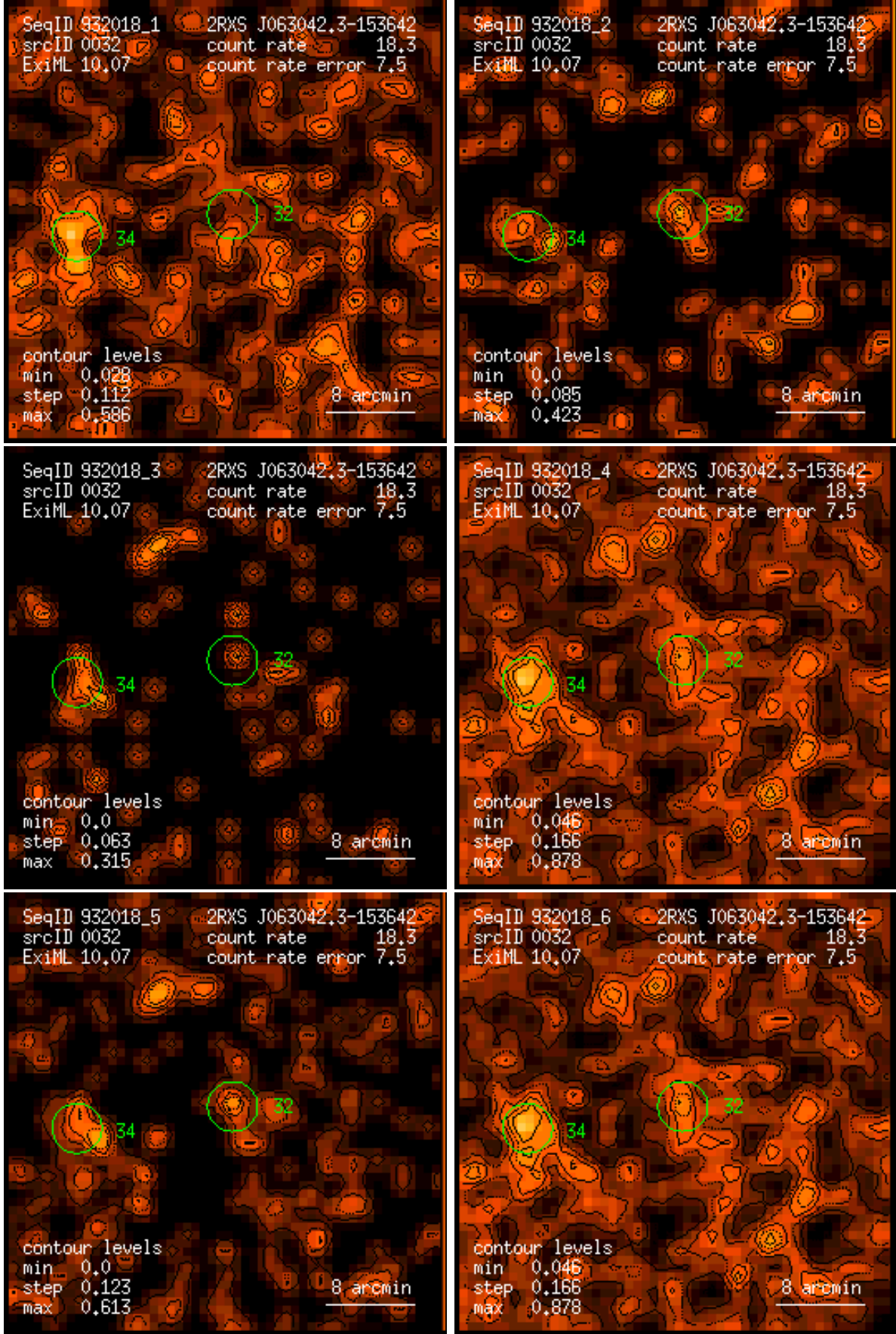
Figure 32: RASS 932018: detection 0032: band rate images, Gaussian filter: (1) PSPC channels 11 – 41, (2) 52 – 90, (3) 91 – 201, (4) 11 – 235, (5) 52 – 201, (6) 11 – 201. Broad band rates in counts/ks. Band rate contour levels in counts/ks/arcmin 2 .
