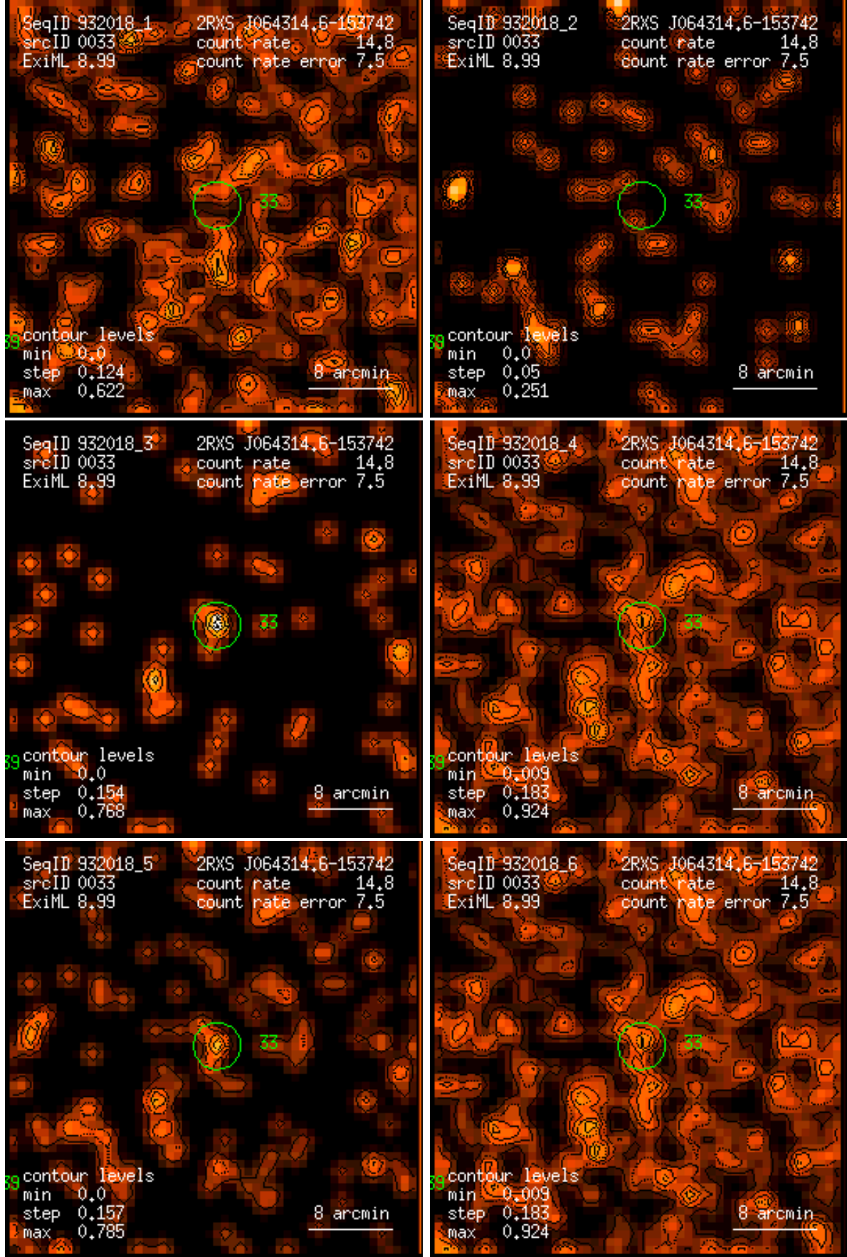
Figure 33: RASS 932018: detection 0033: band rate images, Gaussian filter: (1) PSPC channels 11 – 41, (2) 52 – 90, (3) 91 – 201, (4) 11 – 235, (5) 52 – 201, (6) 11 – 201. Broad band rates in counts/ks. Band rate contour levels in counts/ks/arcmin 2 .
