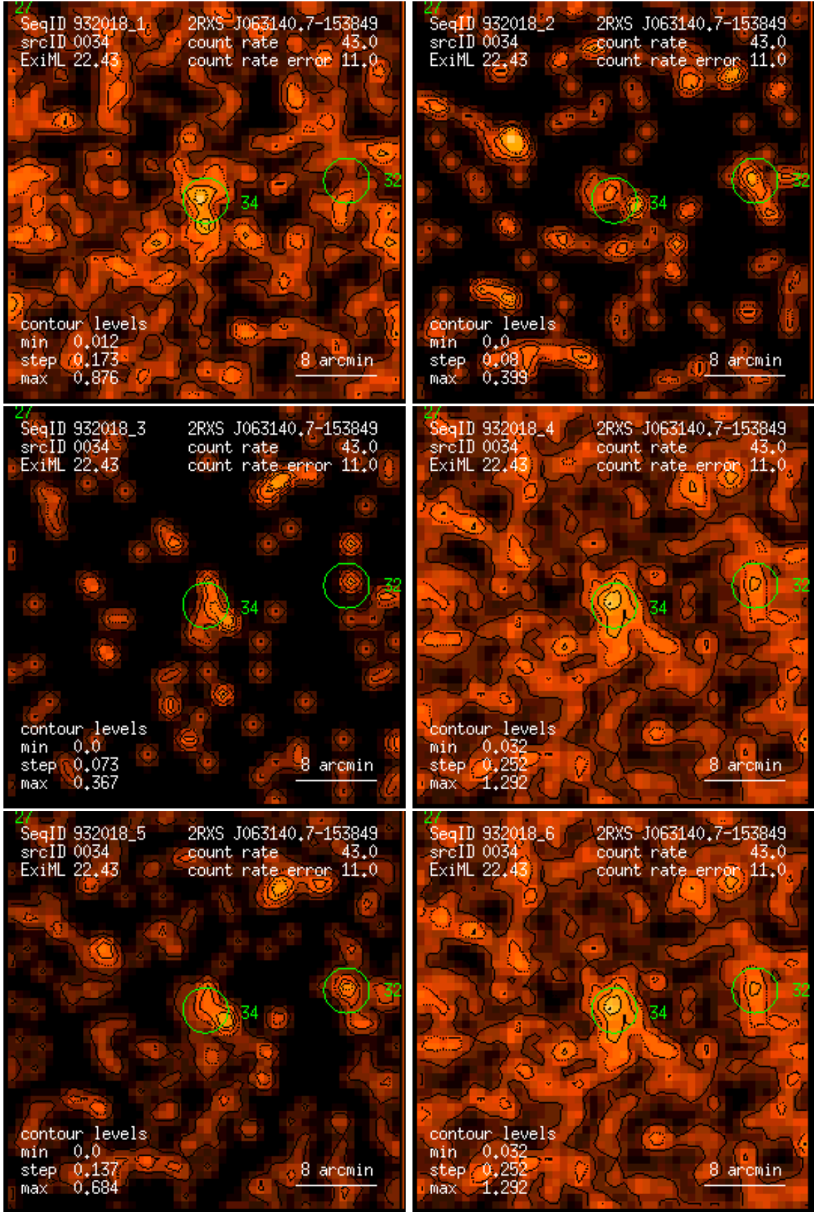
Figure 34: RASS 932018: detection 0034: band rate images, Gaussian filter: (1) PSPC channels 11 – 41, (2) 52 – 90, (3) 91 – 201, (4) 11 – 235, (5) 52 – 201, (6) 11 – 201. Broad band rates in counts/ks. Band rate contour levels in counts/ks/arcmin 2 .
