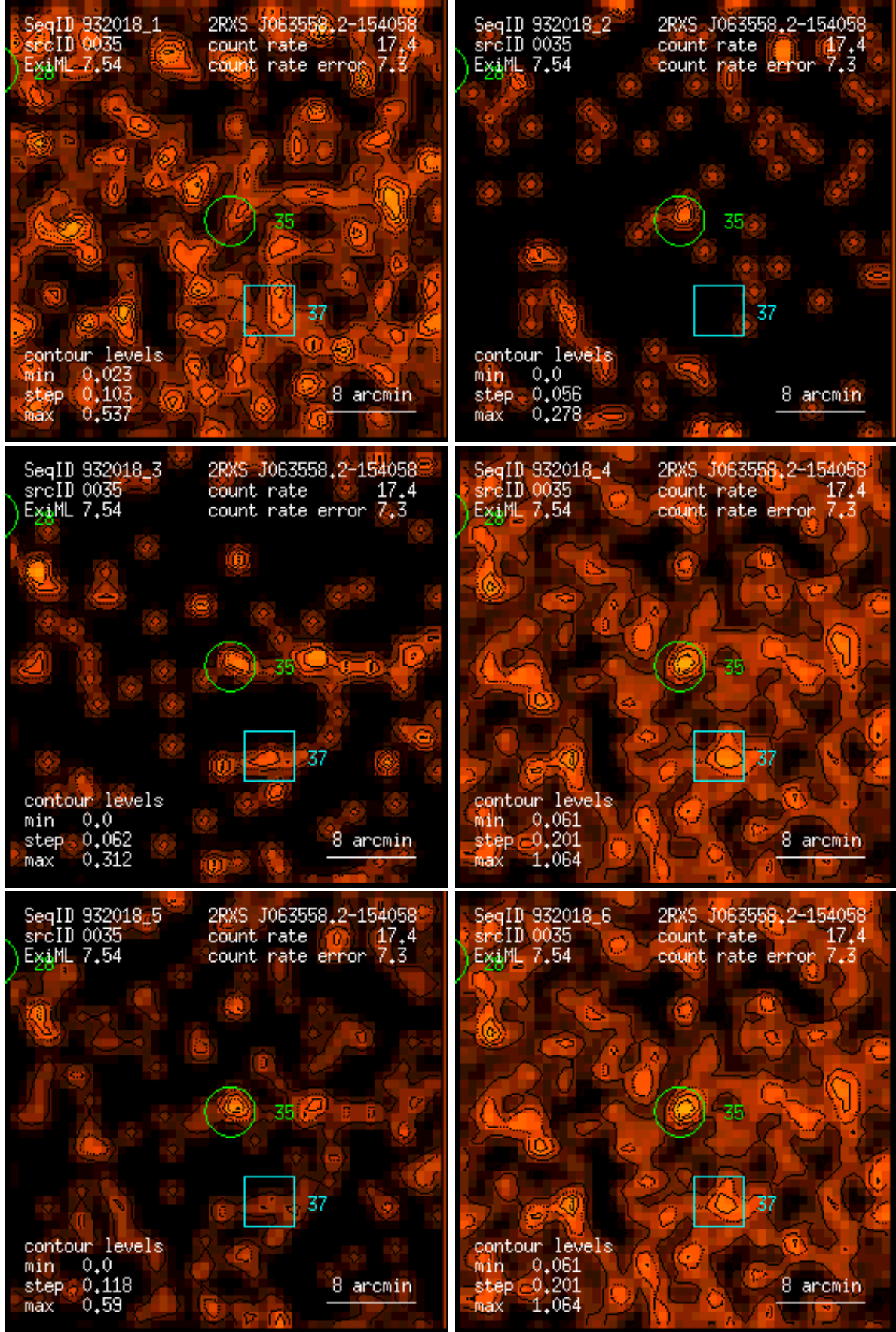
Figure 35: RASS 932018: detection 0035: band rate images, Gaussian filter: (1) PSPC channels 11 – 41, (2) 52 – 90, (3) 91 – 201, (4) 11 – 235, (5) 52 – 201, (6) 11 – 201. Broad band rates in counts/ks. Band rate contour levels in counts/ks/arcmin 2 .
