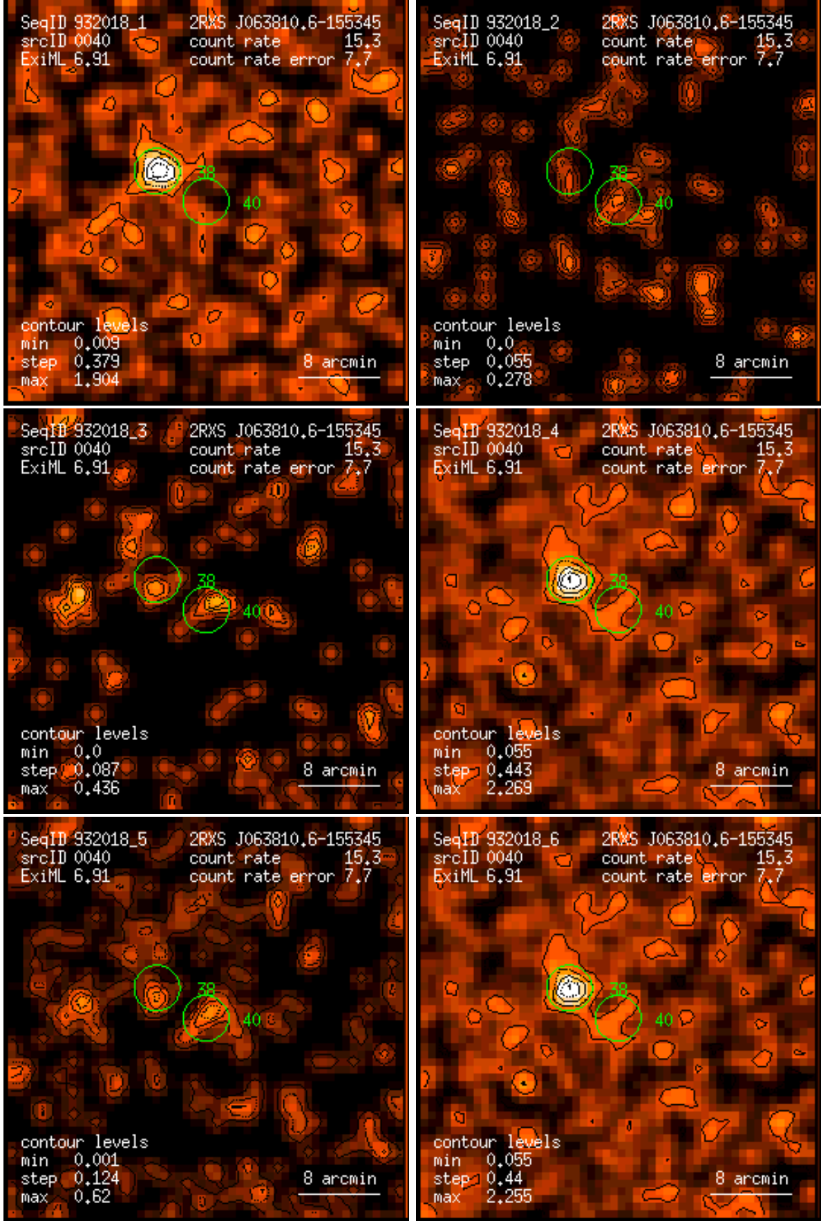
Figure 40: RASS 932018: detection 0040: band rate images, Gaussian filter: (1) PSPC channels 11 – 41, (2) 52 – 90, (3) 91 – 201, (4) 11 – 235, (5) 52 – 201, (6) 11 – 201. Broad band rates in counts/ks. Band rate contour levels in counts/ks/arcmin 2 .
