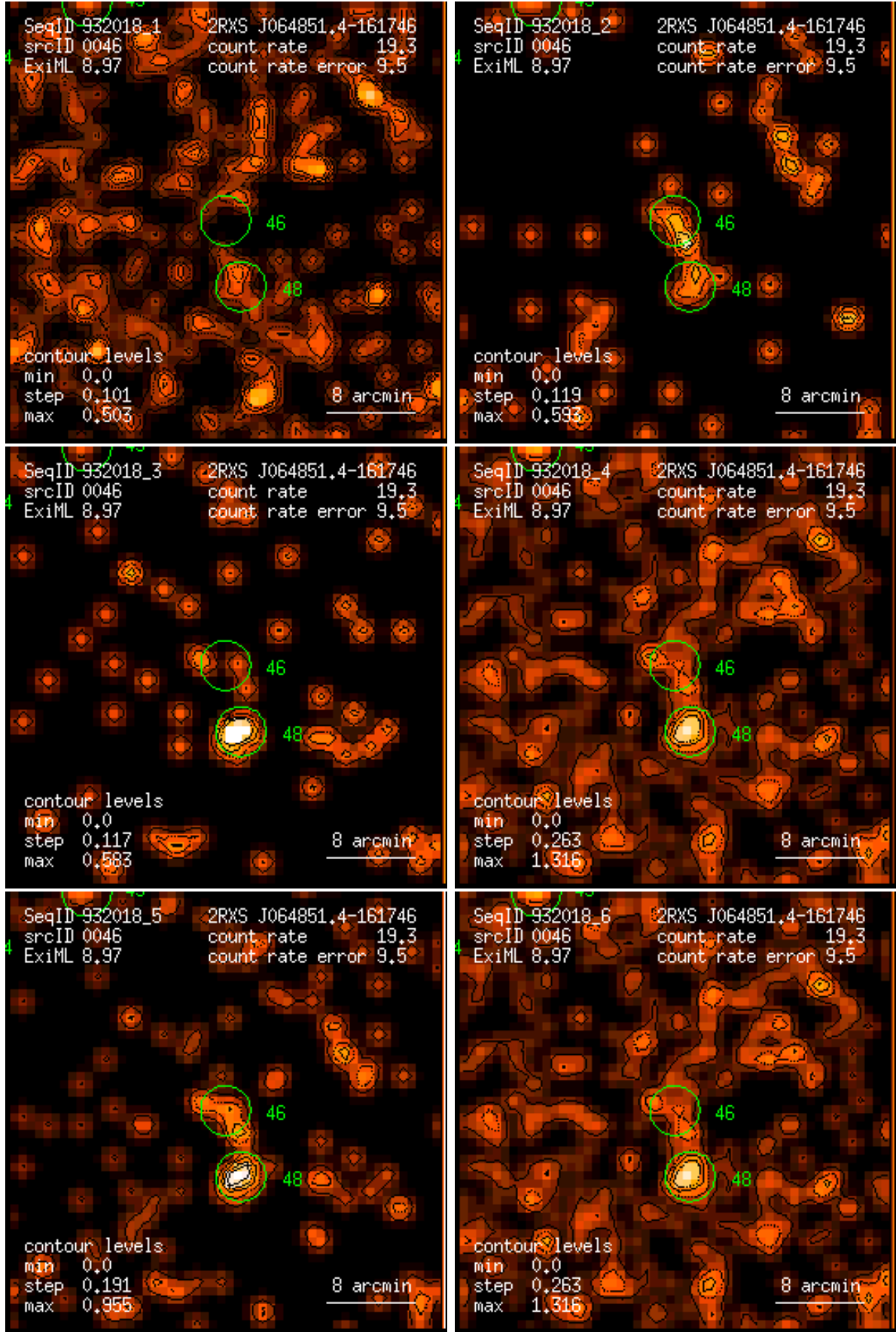
Figure 46: RASS 932018: detection 0046: band rate images, Gaussian filter: (1) PSPC channels 11 – 41, (2) 52 – 90, (3) 91 – 201, (4) 11 – 235, (5) 52 – 201, (6) 11 – 201. Broad band rates in counts/ks. Band rate contour levels in counts/ks/arcmin 2 .
