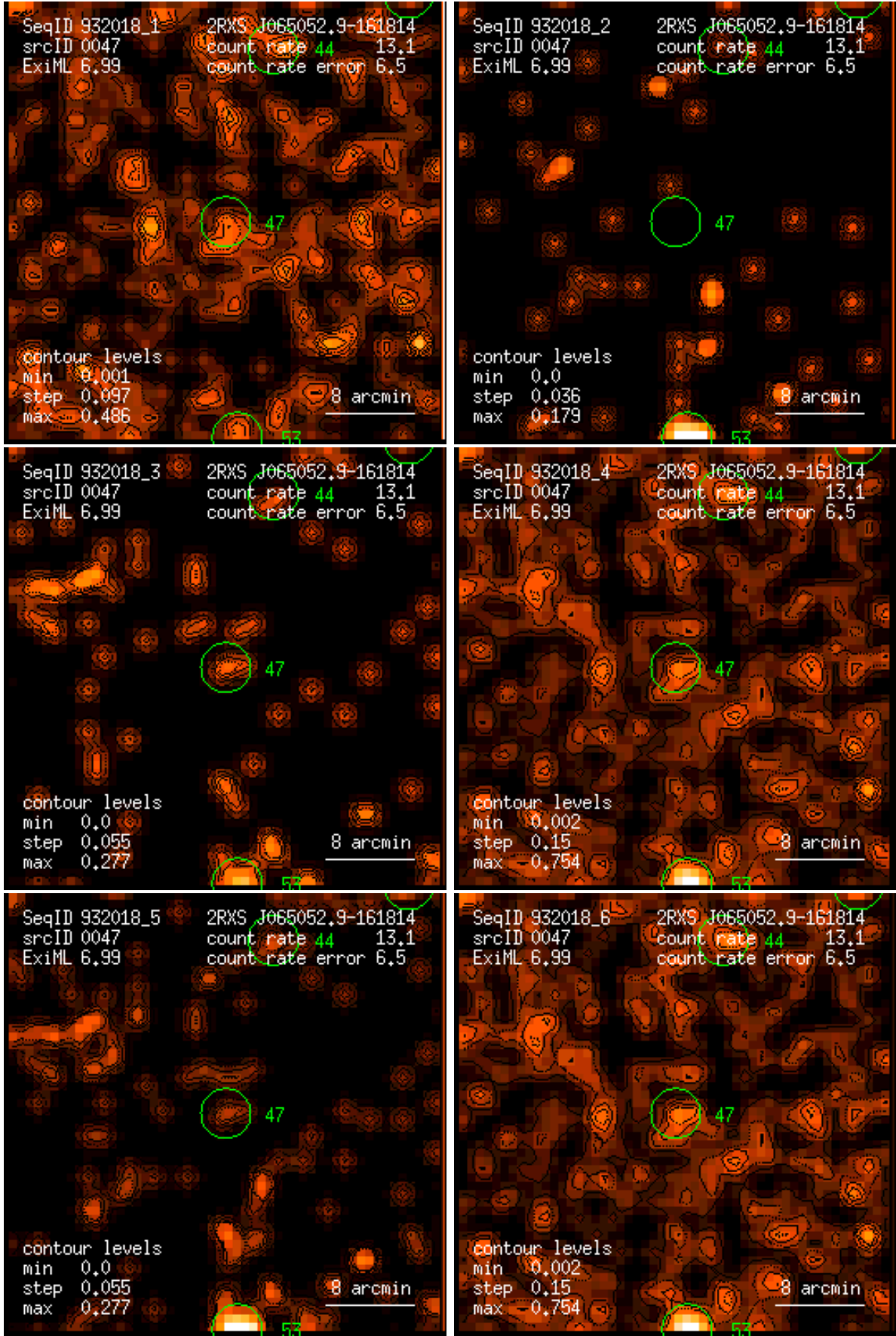
Figure 47: RASS 932018: detection 0047: band rate images, Gaussian filter: (1) PSPC channels 11 – 41, (2) 52 – 90, (3) 91 – 201, (4) 11 – 235, (5) 52 – 201, (6) 11 – 201. Broad band rates in counts/ks. Band rate contour levels in counts/ks/arcmin 2 .
