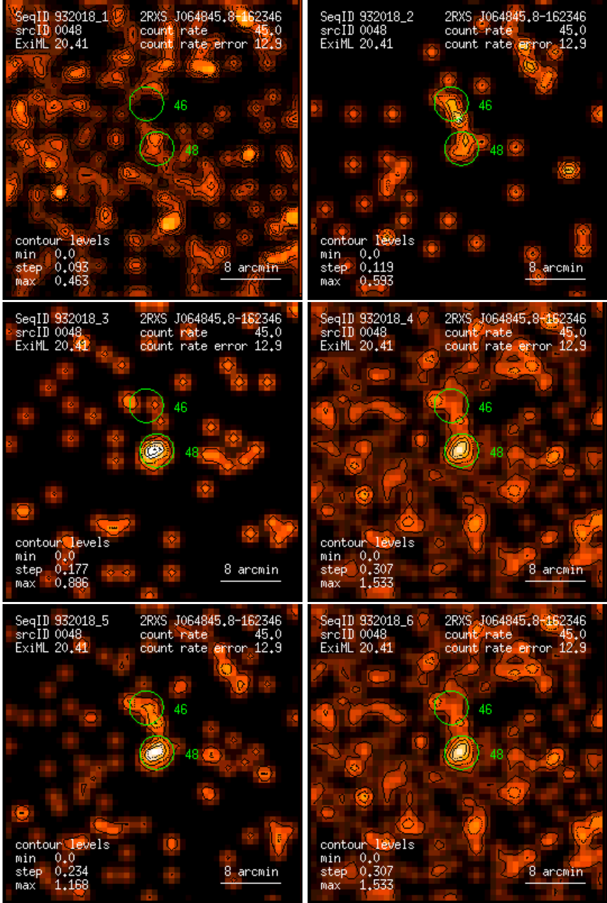
Figure 48: RASS 932018: detection 0048: band rate images, Gaussian filter: (1) PSPC channels 11 – 41, (2) 52 – 90, (3) 91 – 201, (4) 11 – 235, (5) 52 – 201, (6) 11 – 201. Broad band rates in counts/ks. Band rate contour levels in counts/ks/arcmin 2 .
