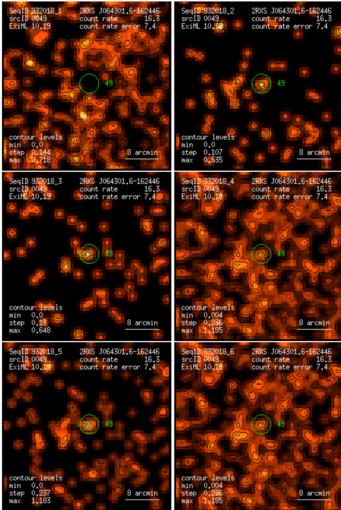
Figure 49: RASS 932018: detection 0049: band rate images, Gaussian filter: (1) PSPC channels 11 – 41, (2) 52 – 90, (3) 91 – 201, (4) 11 – 235, (5) 52 – 201, (6) 11 – 201. Broad band rates in counts/ks. Band rate contour levels in counts/ks/arcmin 2 .
