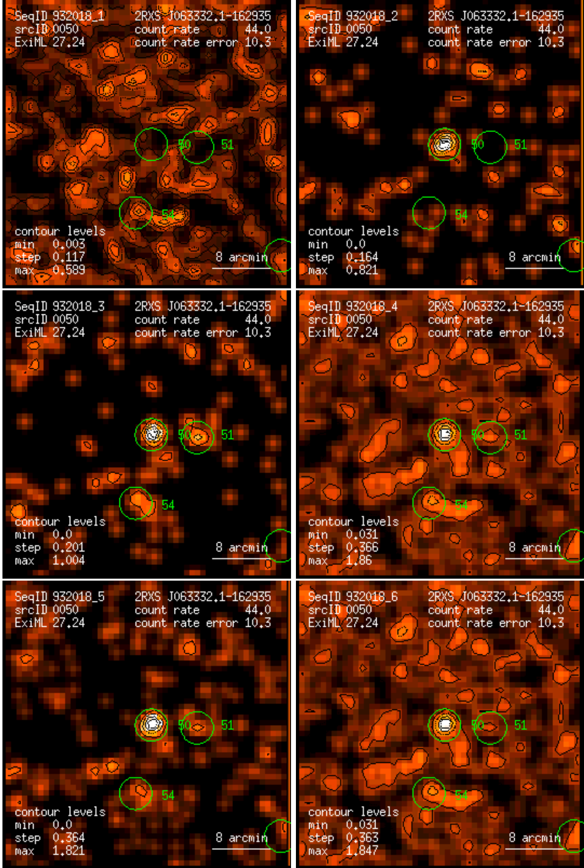
Figure 50: RASS 932018: detection 0050: band rate images, Gaussian filter: (1) PSPC channels 11 – 41, (2) 52 – 90, (3) 91 – 201, (4) 11 – 235, (5) 52 – 201, (6) 11 – 201. Broad band rates in counts/ks. Band rate contour levels in counts/ks/arcmin 2 .
